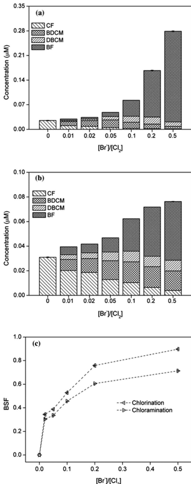
Fig. 5 Effect of bromide on THMs formation from chlorination (a) or chloramination (b) of PBS and corresponding bromine substitution factor (BSF) (c).
