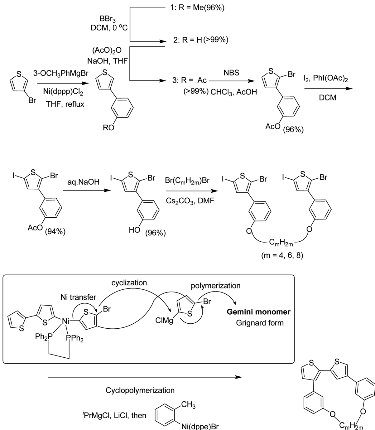
Scheme 20 Proposed cyclopolymerization mechanism based on catalyst-transfer polycondensation.
