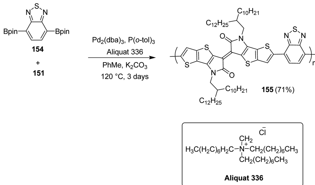
Scheme 49 Copolymerisation of a dibrominated iTT monomer with benzothiadiazole 154 to afford polymer 155 .
