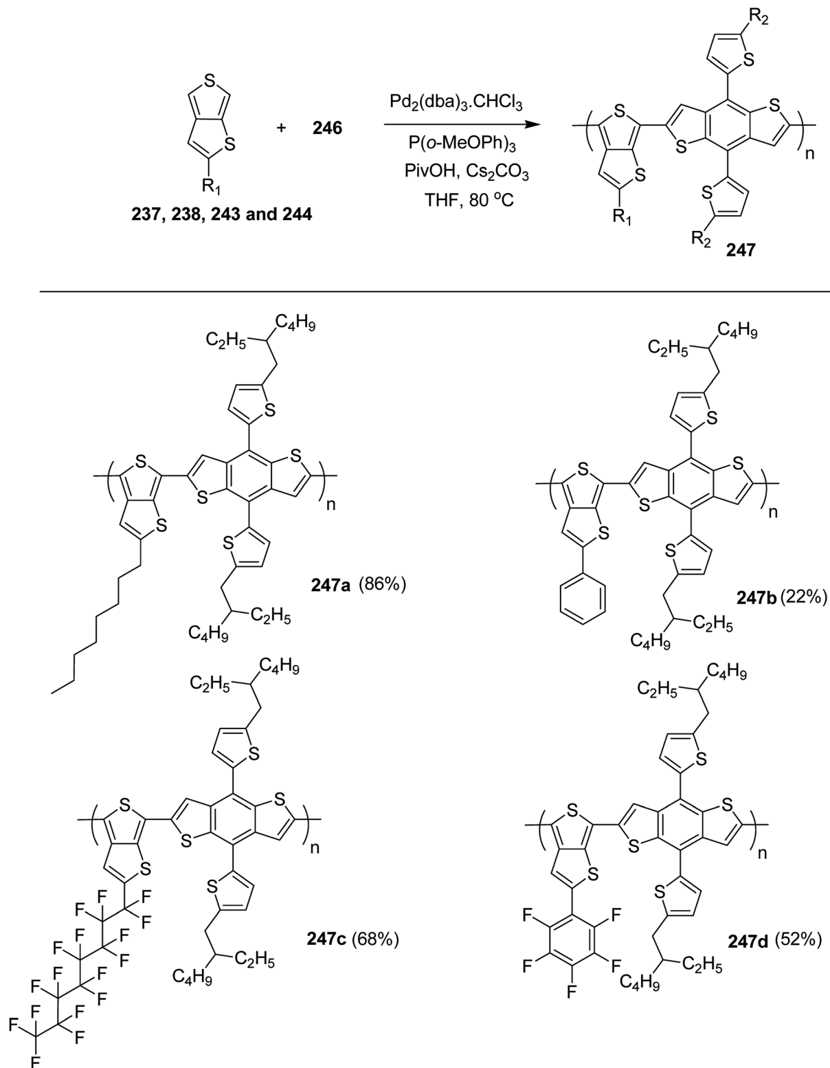
Scheme 72 Synthesis of polymers 247a–d.
