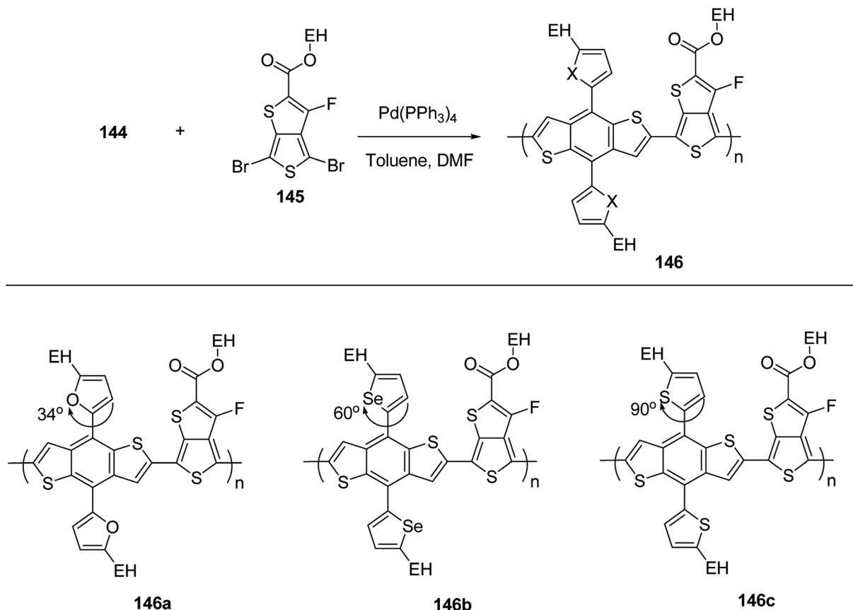
Scheme 46 Synthesis and molecular structures of the polymers 146a–c.
