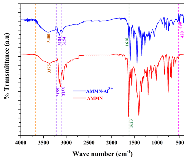
Fig. 9 FT-IR spectrum of AMMN and AMMN- \text{Al}^{3+} complex.
