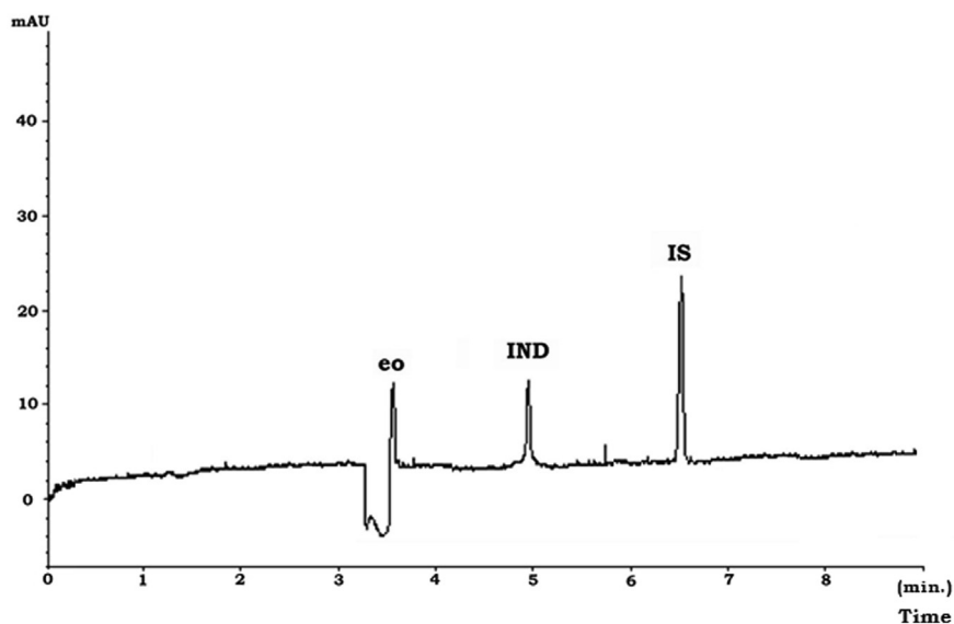
Fig. 3 – A typical electropherogram of Arcapta® capsule on optimum conditions.
