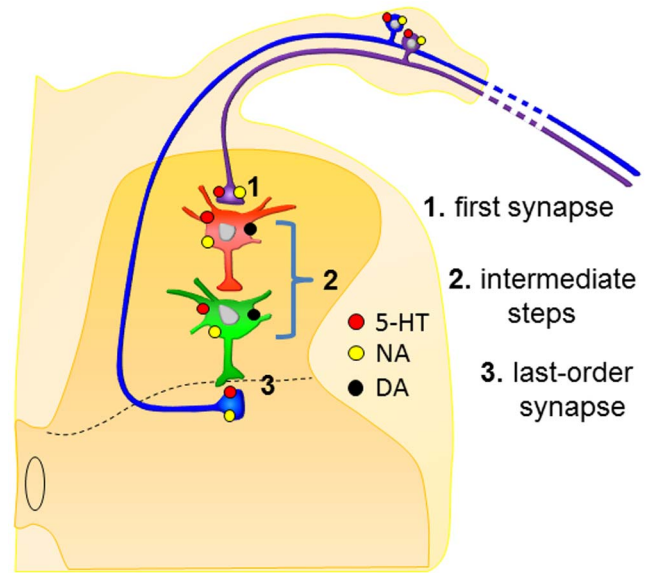
Figure 9. Summary interpretation of changes observed. Drawing highlights putative sites of action of the monoamine transmitters. 1. The short-latency EFP reflects monosynaptic transmission from primary afferents, which is reduced by 5HT and NA, but not DA. As this occurs in the absence of changes in excitability of primary afferents (no change in CAP amplitude), actions are likely exerted via activation of 5HT and NA metabotropic receptors (red and yellow dots, respectively). These receptors will act on signal transduction pathways to reduce synaptic transmission and/or reduce glutamate receptor responsiveness on postsynaptic interneurons. 2. The intraspinal circuit responsible for PAD may involve one or more interposed interneurons, as depicted in the schematic. Monoamines may reduce the excitability of these interneurons and/or reduce transmission between first and higher-order interneurons by activation of 5HT, NA and DA receptors (red, black and yellow dots, respectively) so that fewer interneurons are recruited to produce PAD. 3. 5HT, DA, and NA may act at the last order GABAergic axo-axonic synapse leading to reduced activation of the \text{GABA}_A -like receptors responsible for producing PAD. doi:10.1371/journal.pone.0089999.g009
