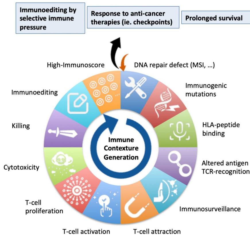
Figure 1. DNA repair defect, tumor immune contexture and prognosis. Colorectal cancers (CRCs) with microsatellite instability (MSI) are due to a defect of the DNA mismatch repair (MMR) system that leads to an accumulation of insertions and deletions of nucleotides into repeat sequences. When such mutations occur in coding sequences, reading frames of the genes can be shifted and neo-antigens synthesized and presented at the surface of the mutated tumor cells, as neo-peptides bound to HLA-I molecules. These antigens can be considered as non-self and elicit immune reactions. T-cells can then be attracted to the tumor site and stimulated for proliferation and cytotoxic activity. Tumor cells harboring such immunogenic mutation can then be exposed to a selective immune pressure, the tumor immunoediting. Such anti-immune responses, characterized by high immune infiltrations (high Immunoscore) are associated with better clinical outcomes and responses to immunotherapies.
