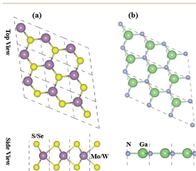
Fig. 1 Top and side view of the free standing (a) MX 2 (M = Mo, W; X = S, Se) and (b) GaN monolayers.
