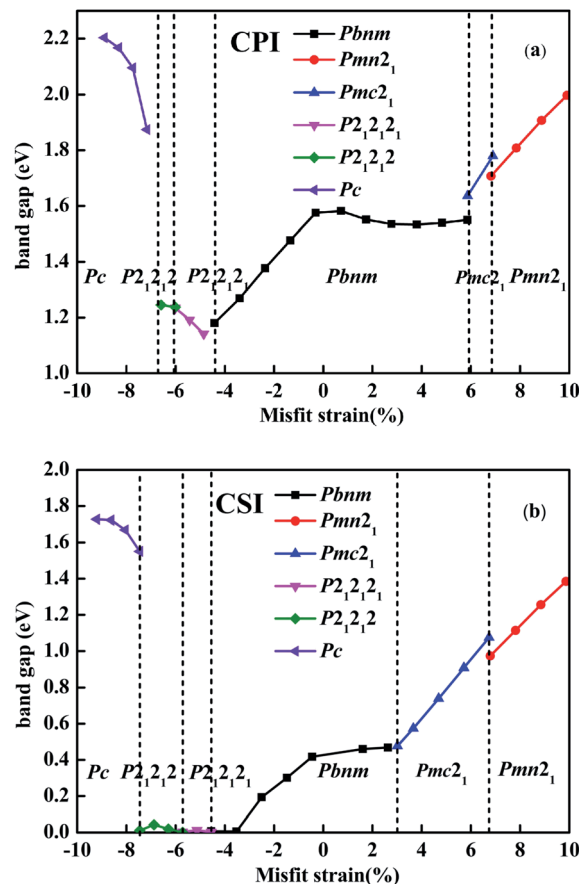
Fig. 4 Band gaps of different stable phases vs. misfit strain of CPI and CSI, respectively.
