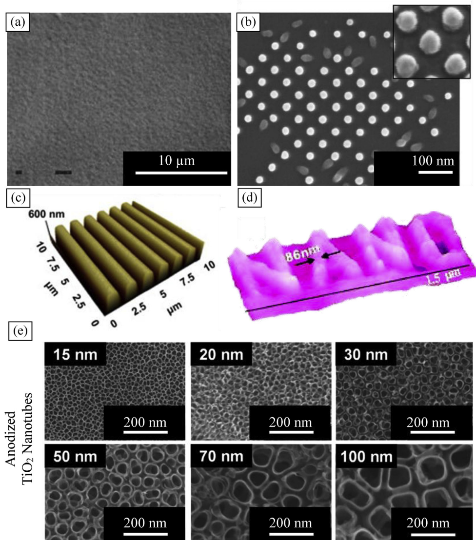
Fig. 1. Morphologies of representative nanostructured surfaces. (a) Nanorough poly-ether-urethane surface fabricated by alkaline chemical etching using NaOH (adapted from Ref. [44] with permission by John Wiley and Sons). (b) 50 nm-periodic array of nanoscale Co/Pd-coated \text{SiO}_x islands fabricated by extreme ultraviolet interference lithography (Reprinted from Ref. [47] (Luo F, Heyderman L, Solak H, Thomson T, Best M, Nanoscale perpendicular magnetic island arrays fabricated by extreme ultraviolet interference lithography . Applied Physics Letters 2008; 92:102505.) with the permission of AIP publishing. (c) Nanopatterned parallel grooves on the surface of PLGA (50:50) with 800 nm ridge width and 800 nm groove width, fabricated by capillary force lithography [40] (reprinted from Biomaterials, 2014. 35(5), Yang HS, Ieronimakis N, Tsui JH, Kim HN, Suh K-Y, Reyes M et al., Nanopatterned muscle cell patches for enhanced myogenesis and dystrophin expression in a mouse model of muscular dystrophy . p. 1478–1486. Copyright (2017), with permission from Elsevier). (d) 3D image of nanopatterned “NANO” made of cross-linked carbozole drawn on a film of precursor polycarbozole, imaged using an atomic force microscope. (adapted and reprinted with permission from Ref. [58] (Jegadesan S, Sindhu S, Advincula RC, Valiyaveetil S, Direct electrochemical nanopatterning of polycarbozole monomer and precursor polymer films: ambient formation of thermally stable conducting nanopatterns . Langmuir, 2006. 22(2): p. 780–786.). Copyright (2017) American Chemical Society. (e) Anodized \text{TiO}_2 nanotubes with six different pore sizes from 15 nm to 100 nm (adapted and reprinted with permission from Ref. [14] (Park J, Bauer S, von der Mark K, Schmuki P, Nanosize and vitality: \text{TiO}_2 nanotube diameter directs cell fate . Nano letters, 2007. 7(6): p. 1686–1691.). Copyright (2017) American Chemical Society.). Scale bar = 10 \mu\text{m} for (a), 100 nm for (b), 1.5 \mu\text{m} for (d) and 200 nm for (e).
