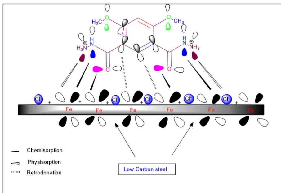
Fig. 11 Schematic figure of LCS corrosion inhibition in a 0.5 \text{ mol L}^{-1} HCl solution in the presence of the DMIH compound.
