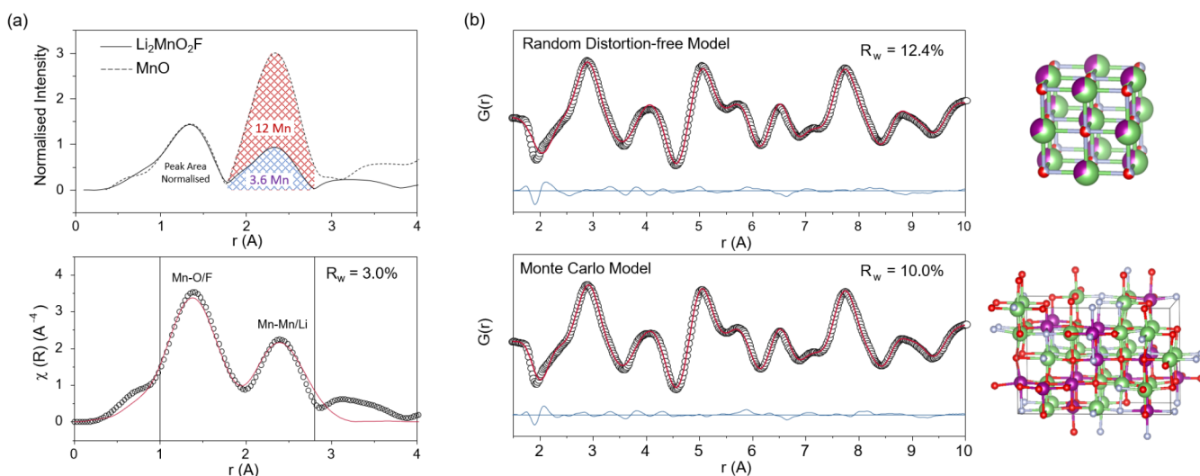
Figure 2. Structure of \text{Li}_2\text{MnO}_2\text{F} . (a) Mn K-edge EXAFS for pristine \text{Li}_2\text{MnO}_2\text{F} compared with a MnO reference, each with cubic rocksalt crystal structure. The spectra are normalized to the area under the first peak corresponding to the occupancy of the first nearest neighbor anion site which is the same for both, 6. A good fit of the EXAFS data can also be obtained with a rocksalt model with 4 \times 2 nearest neighbor Mn. (b) Neutron PDF data fitted to structural models of distortion-free random cubic rocksalt and the Monte Carlo derived model for pristine \text{Li}_2\text{MnO}_2\text{F} . Li, Mn, O, and F atoms are indicated by green, purple, red, and gray spheres, respectively. There is very good agreement between the models and the PDF data showing \text{Li}_2\text{MnO}_2\text{F} exhibits a close to completely disordered rocksalt structure. The slight asymmetry of the first peak at around 1.9 \text{ \AA} may indicate some element-specific preference for shorter bond length. Refined cell parameters a = 4.117 \text{ \AA} and a = 12.152 \text{ \AA} , b = c = 8.336 \text{ \AA} , and U_{\text{iso}} values 0.027 and 0.014, respectively.
