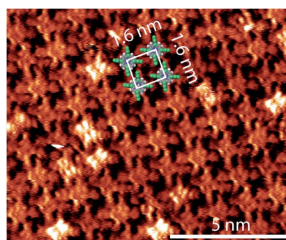
Fig. 4 2HTFPP after annealing to 200\text{ }^\circ\text{C} . The unit cell has dimensions of 1.6\text{ nm} \times 1.6\text{ nm} and the monolayer has a packing density of 0.38 molecules per \text{nm}^2 . The bright double-dot features are doubly stacked porphyrins, the start of a second layer. The image was taken with a bias voltage of -10.0\text{ mV} and a tunneling current of 10\text{ pA} .
