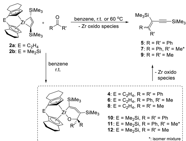
Scheme 3 Reaction of complexes 2a and 2b with ketones to yield enynes 5, 7 and 9. Note: compound 4 contains compound 13 ( vide infra ) as an impurity as 2a, used for its synthesis always contains traces of 3a (Fig. S43†).
