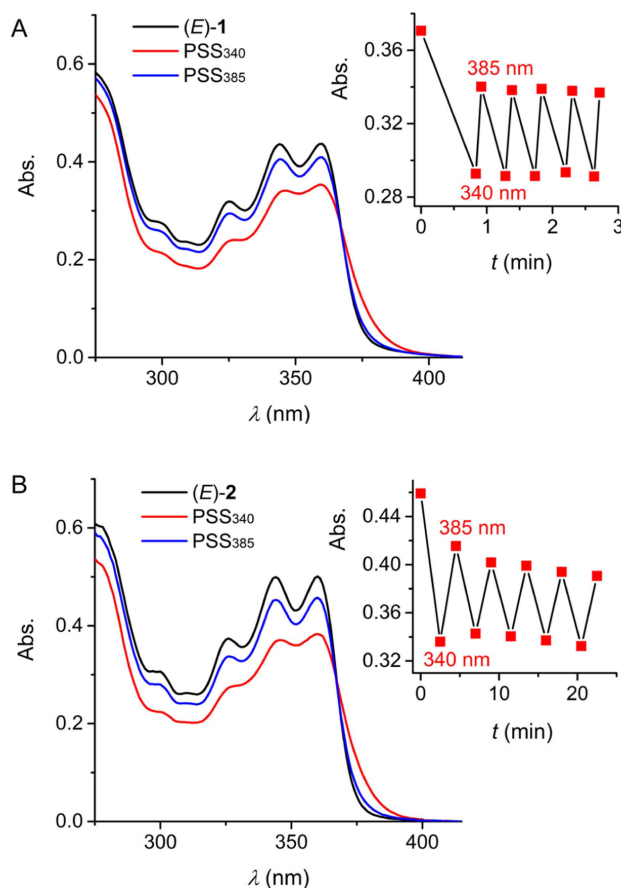
Figure 2. UV/Vis spectral changes starting from ( E )- 1 (A) and ( E )- 2 (B) upon 340 nm irradiation followed by 385 nm irradiation ( c=2 \times 10^{-5} M in degassed DMSO). The insets show 340/385 nm irradiation cycles.
