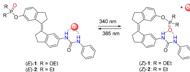
Scheme 1. Photocontrolled anion binding and release by blockage of the urea binding site through intramolecular hydrogen bonding.
