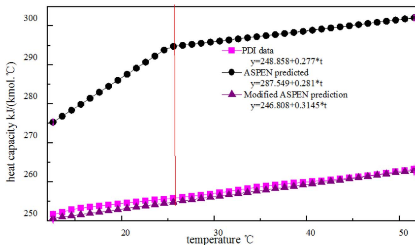
Fig. 4 Plots of the heat capacity of temperature for PDI experimental data, Aspen predicted and modified Aspen prediction model.
