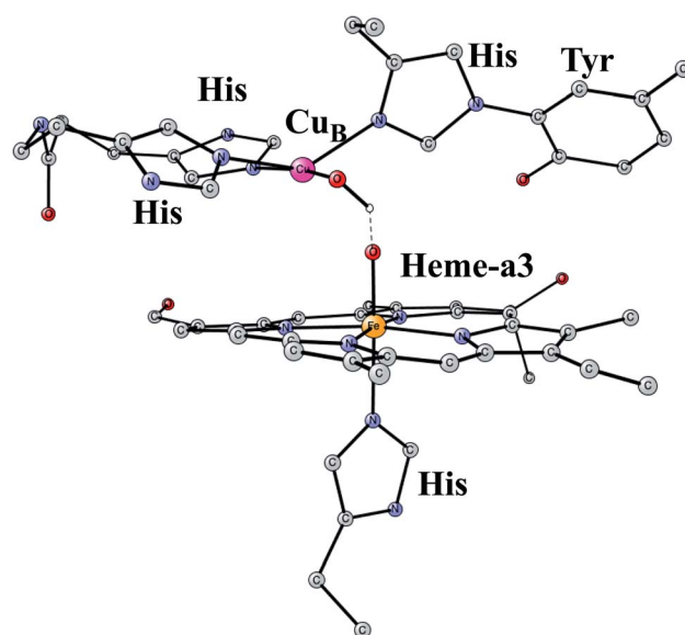
Fig. 3 An optimized structure of the active site of CcO, obtained after the cleavage of the O–O bond of O_2 .
