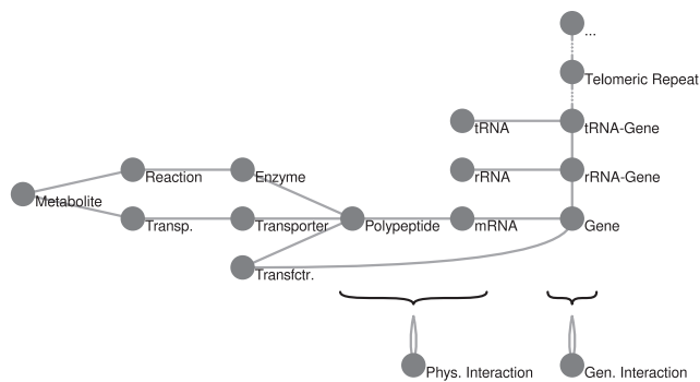
Fig. 1. Simplified schematic of the data structure underlying the Ondex Saccharomyces knowledge network. Circles represent concept types, and lines represent relations between them.
