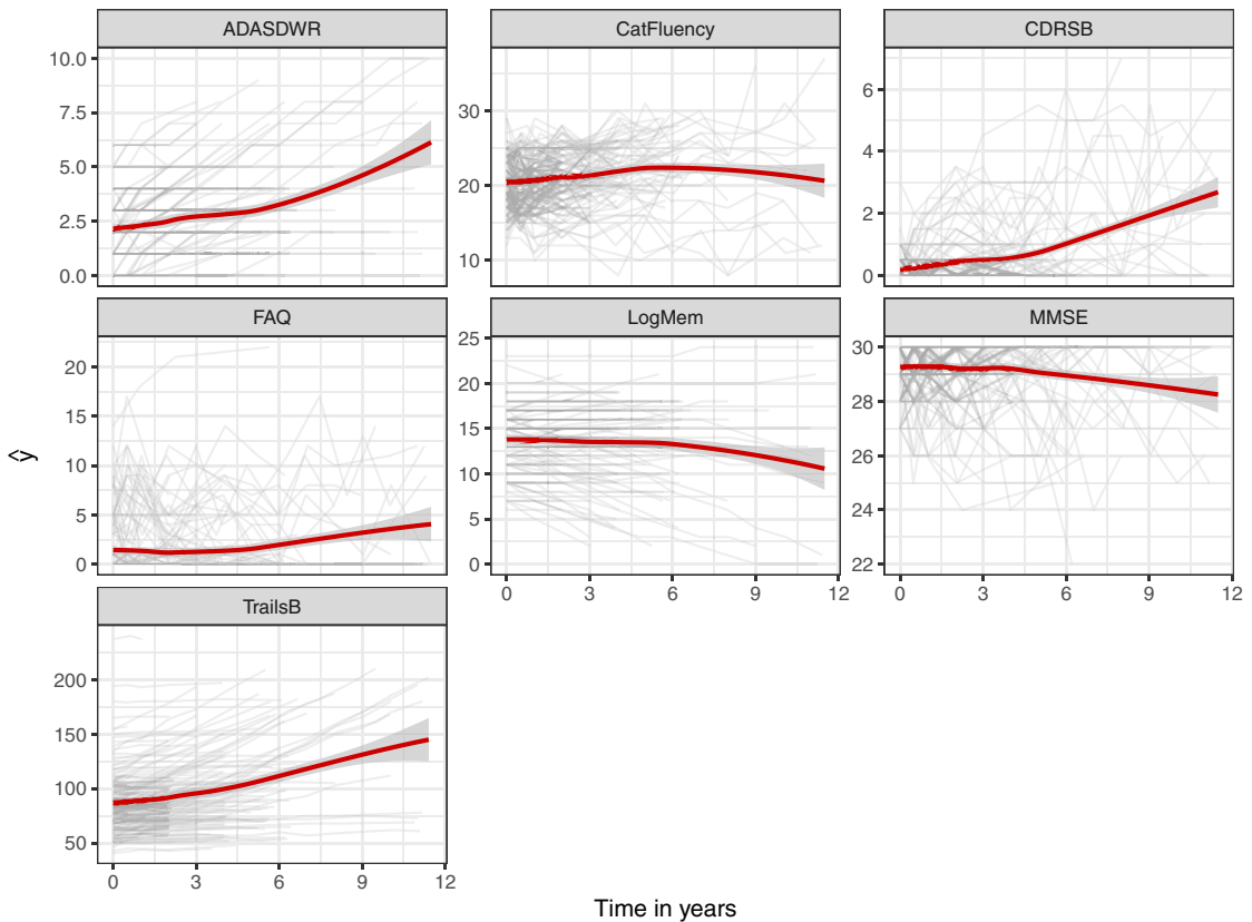
Fig. 1. Observed (upper panel) and predicted (lower panel) longitudinal profiles of the seven markers for all individuals. Bold lines are locally estimated scatter plot smoother. Abbreviations: ADASDWR, Alzheimer's Disease Assessment Scale delayed word recall; MMSE, Mini-Mental State Examination; CDRSB, Clinical Dementia Rating—Sum of Boxes; FAQ, functional assessment questionnaire.
