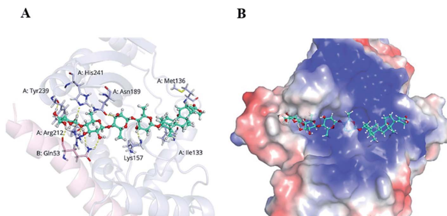
Fig. 10 Docking analysis of 1 with VASH2. (A) Amino acid residues of VASH2 with close proximity to 1 . (B) Space-filling model of VASH2 with its potential ligand 1 .
