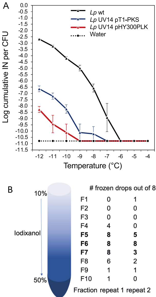
Fig. 3 Complementation of a T1-PKS UV-mutant and results from gradient ultracentrifugation of the LINA particle. A Freezing spectra based on three replicates of droplet freezing assays (using 30 drops per dilution per replicate) of Lp VT1065 wild-type ( Lp wt), Lp mutant UV14 with two SNPs in the T1-PKS gene containing the empty vector pHY300PLK, and Lp mutant UV14 complemented with plasmid pHY300PLK containing the T1-PKS gene (pT1-PKS). The X-axis shows the temperature and Y-axis shows the concentration of ice nucleation particles (INP) per colony forming unit (CFU). B The LINA particle was separated from Lp VT1065 cells and concentrated by differential filtration in a iodixanol gradient and then subjected to gradient ultracentrifugation. Samples from the indicated fractions were diluted 1:100 (to reduce the concentration of iodixanol) and analyzed by a droplet freezing assay at -11^{\circ}\text{C} (at which the difference in the number of frozen droplets was the highest). The whole experiment was repeated twice. The number of frozen droplets out of a total of 8 droplets per fraction is listed.
