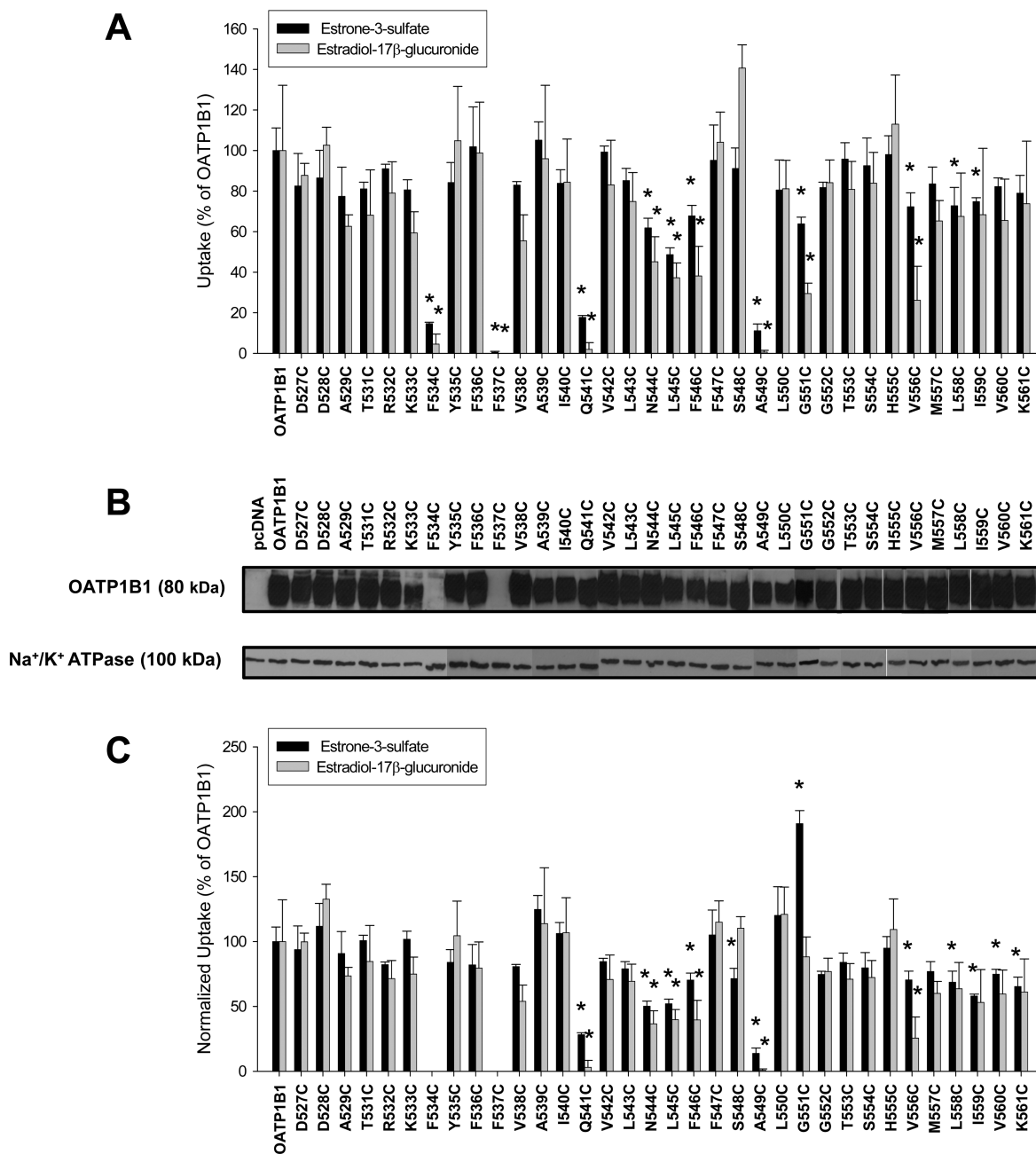
Figure 2. Substrate transport and surface expression of OATP1B1 and the TM10 cysteine mutants. (A) Uptake of 0.1 μM [ 3 H]estrone-3-sulfate (black bars) or 1 μM [ 3 H]estradiol-17β-glucuronide (gray bars) was measured with HEK293 cells transfected with empty vector, OATP1B1, or 34 cysteine mutants at 37 °C for 30 s (estrone-3-sulfate) or 2 min (estradiol-17β-glucuronide), respectively. After the values obtained with empty vector transfected cells were subtracted, results were calculated as a percentage of uptake activity for OATP1B1. Each bar is the mean ± SD of three individual experiments. An asterisk (*) indicates values significantly different from that of OATP1B1 ( p < 0.05). The amino acid on the left side (D527) is located close to the predicted extracellular side of TM10, while the one on the right side (K561) is located at the predicted cytoplasmic side of TM10. (B) Biotinylated membrane proteins were subjected to Western blot analysis with an anti-His antibody detecting the C-terminal end of OATP1B1 and the mutant proteins. The plasma membrane marker Na + /K + ATPase α subunit was used as protein loading control. (C) Uptake values shown in (A) were corrected for protein expression and are given as normalized uptake. Asterisks (*) indicate values significantly different from that of OATP1B1 ( p < 0.05).
