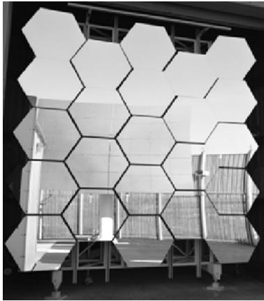
Fig. 1. The 10 kW high-flux solar furnace of the National Renewable Energy Laboratory, Golden, USA.
