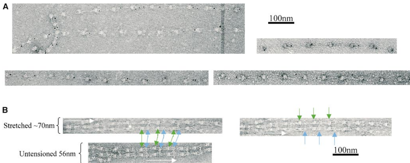
Figure 3. Antibody and gold binding to microfibrils extended by surface tension. (A) Fibrillin-rich microfibrils were extended by surface tension, and then labeled with 5-nm colloidal gold and negatively stained. (B) Negatively stained images of microfibrils labeled with antibody 12A5.18, either unstretched or extended by surface tension. Only extension up to \sim 10 nm is tolerated before the antibody banding pattern is lost. Microfibril direction is indicated by a white arrow, bead position by green arrows, and antibody position is represented by blue arrows.
