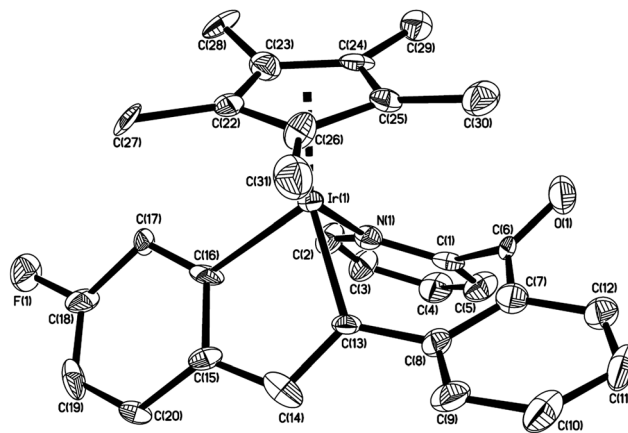
Fig. 2 Thermal ellipsoid drawing of 4c showing the labeling scheme and 30% probability ellipsoids; hydrogens are omitted for clarity. Selected bond lengths [Å] and angles [°] are \text{Ir}(1)\text{--}\text{N}(1) 2.065(12), \text{Ir}(1)\text{--}\text{C}(13) 2.062(12), \text{Ir}(1)\text{--}\text{C}(16) 2.090(13), \text{C}(13)\text{--}\text{C}(14) 1.378(19), \text{C}(8)\text{--}\text{C}(13) 1.455(19), \text{Ir}(1)\text{--}\text{Cp}(\text{centroid}) 1.862, \angle \text{N}(1)\text{--}\text{Ir}(1)\text{--}\text{C}(13) 85.0(5), \angle \text{N}(1)\text{--}\text{Ir}(1)\text{--}\text{C}(16) 88.6(5), \angle \text{C}(13)\text{--}\text{Ir}(1)\text{--}\text{C}(16) 78.3(5), \angle \text{Ir}(1)\text{--}\text{C}(13)\text{--}\text{C}(14) 117.2(11), \angle \text{Ir}(1)\text{--}\text{C}(13)\text{--}\text{C}(8) 121.1(9).
