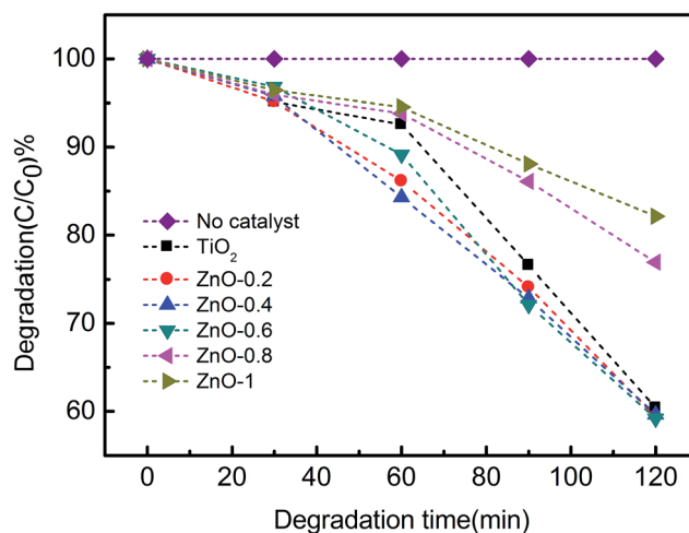
Fig. 5 Degradation kinetics of methyl orange solution by \text{TiO}_2 NTs films and various types of \text{ZnO}@/\text{TiO}_2 heterojunction films.
