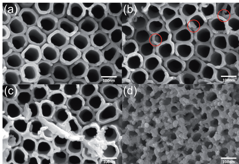
Fig. 3 SEM images of \text{TiO}_2 NTs and \text{ZnO}@/\text{TiO}_2 heterojunctions: (a) \text{TiO}_2 NTs arrays. (b–d) SEM of heterojunctions with zinc acetate at various concentrations: 0.2 \text{ mol L}^{-1} , 0.6 \text{ mol L}^{-1} and 1 \text{ mol L}^{-1} , respectively.
