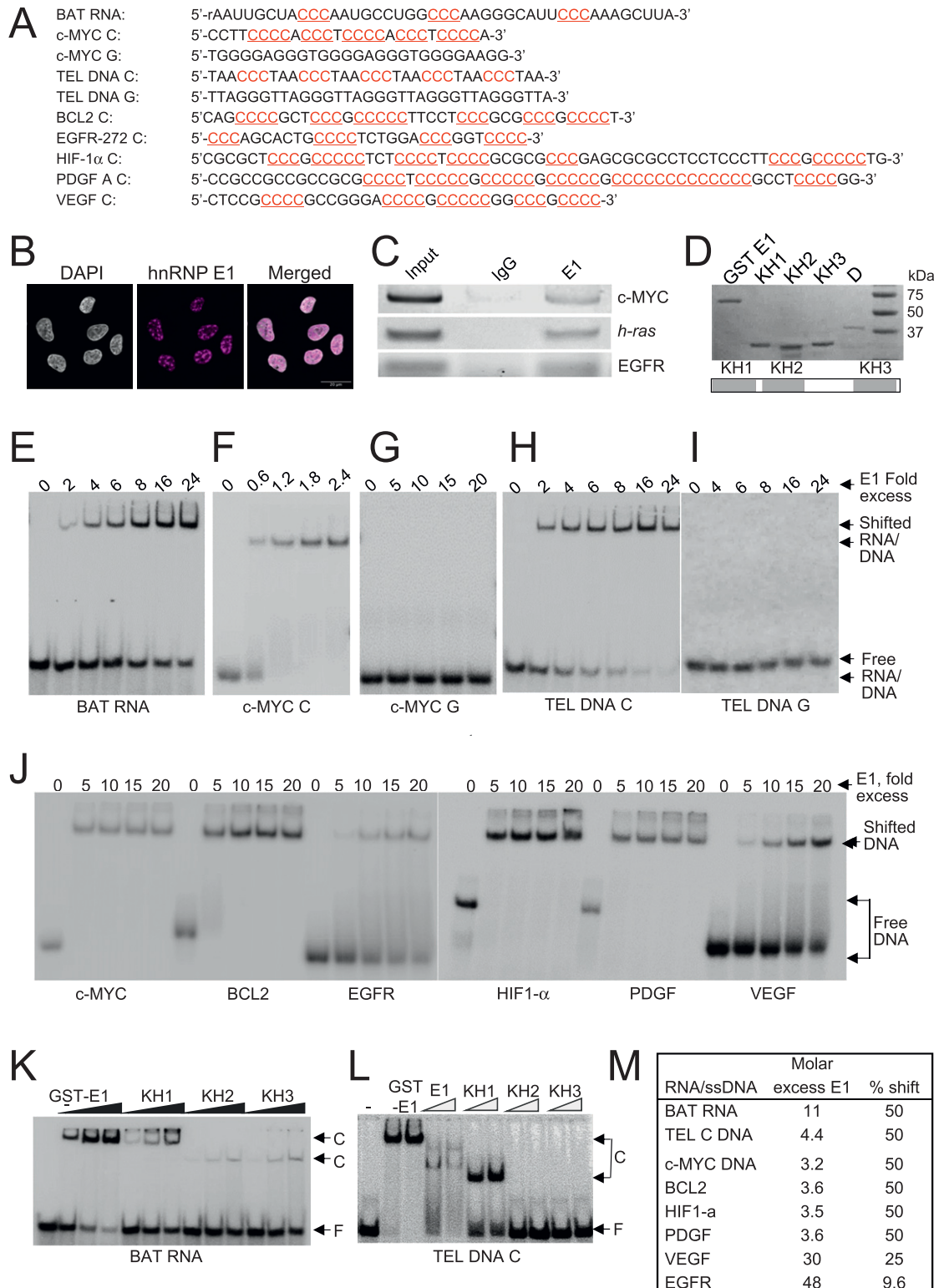
Figure 1. hnRNP E1 binds polycytosine-rich DNA tracts.
