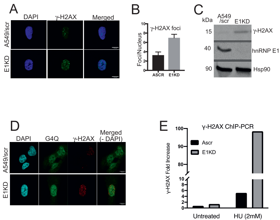
Figure 3. Role of hnRNP E1 in genome integrity. (A, B) Immunofluorescence showing \gamma -H2AX activation in E1KD cells. (C) Western blot showing \gamma -H2AX activation in E1KD cells. (D) Immunofluorescence showing increase in and colocalization of \gamma -H2AX and G4 foci in E1KD cells. (E) ChIP-qPCR analysis showing \gamma -H2AX localization at c-MYC promoter of scrambled (A549) and hnRNP E1 knockdown (E1KD) cells.
