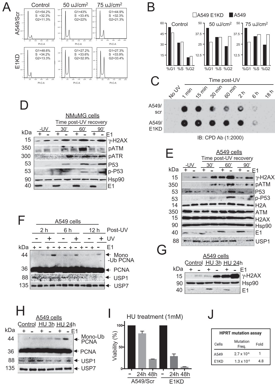
Figure 4. E1KD phenotype acts synergistically with HU/UV and promotes mutation.
