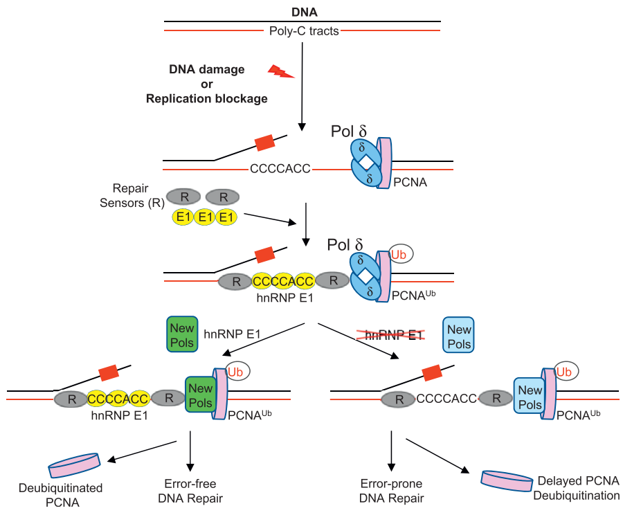
Figure 5. Model showing the role of hnRNP E1 in genome integrity.
