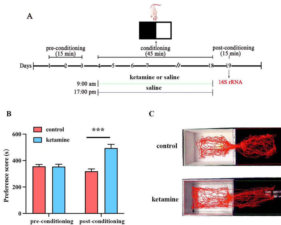
Figure 1 Ketamine induced CPP in mice. (A) The experimental design for CPP testing. (B) Time spent in the white box by mice was measured, showing no differences before establishing the ketamine-induced CPP model. (C) Representative trajectories of mice in the white box during post-conditioning phase with or without ketamine administration. Each bar represents the mean \pm SEM. *** P < 0.001 by unpaired two-tailed Student's t -test.
