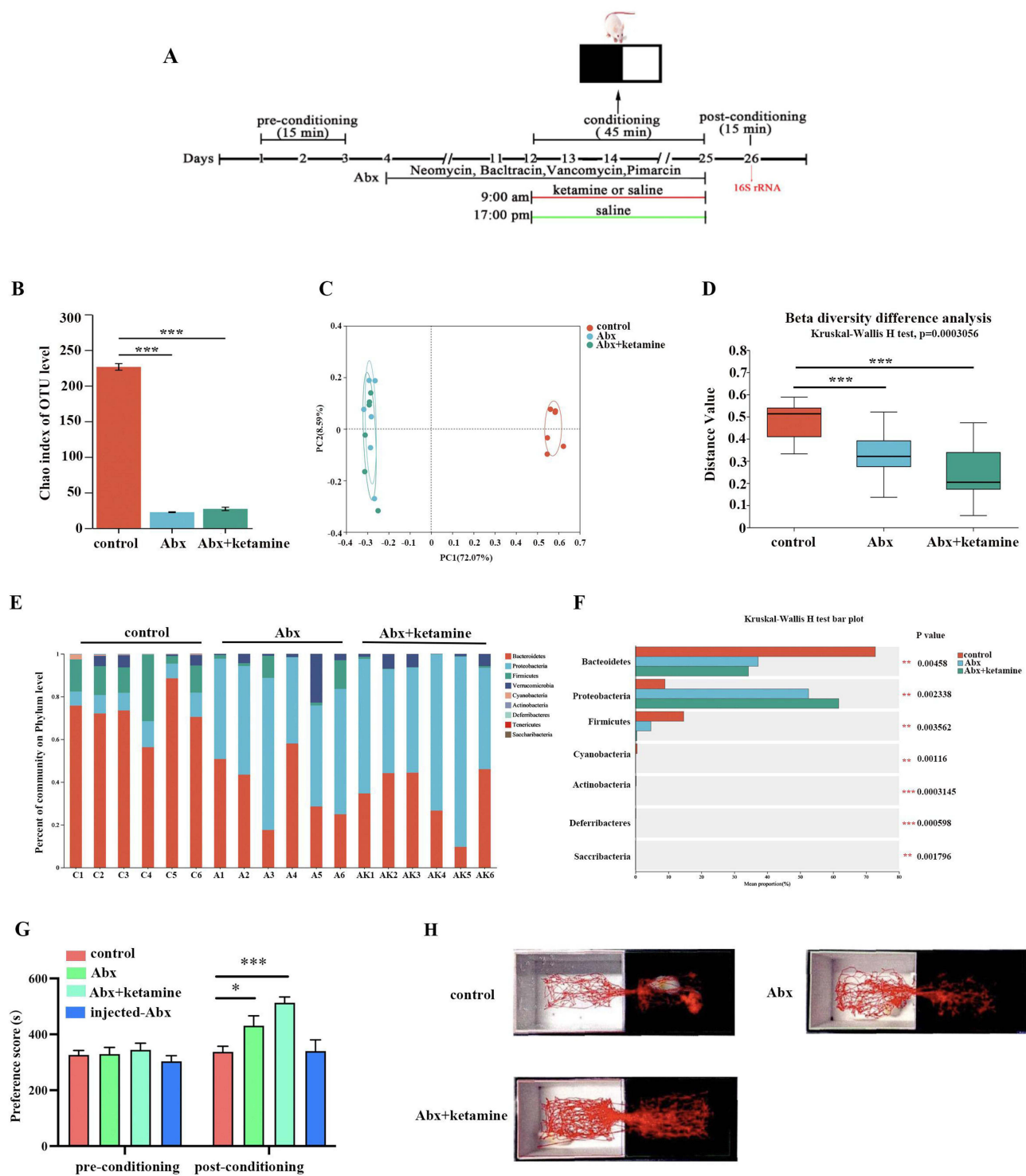
Figure 6 The effect of antibiotic on ketamine addiction. (A) Experimental timeline for the oral antibiotic treatment and CPP training. (B) Chao index for each group ( n = 6 ). (C) PCoA analysis of the microbial communities in each group ( n = 6 ). (D) \beta -diversity analysis of the microbial communities among groups. (E) Composition plot at the phylum level in control, Abx, Abx+ketamine group. (F) Significant differences in the relative abundances of microbes at the phylum level among the groups. (G) The mice were assessed for the time spent in the white box before and after treatment with or without an oral antibiotic cocktail and ketamine ( n = 8 ). (H) Representative trajectories of mice in the white box during the post-conditioning phase. Each bar represents the mean \pm SEM. * P < 0.05 , ** P < 0.01 , *** P < 0.001 by Kruskal–Wallis H -test and one-way ANOVA.
