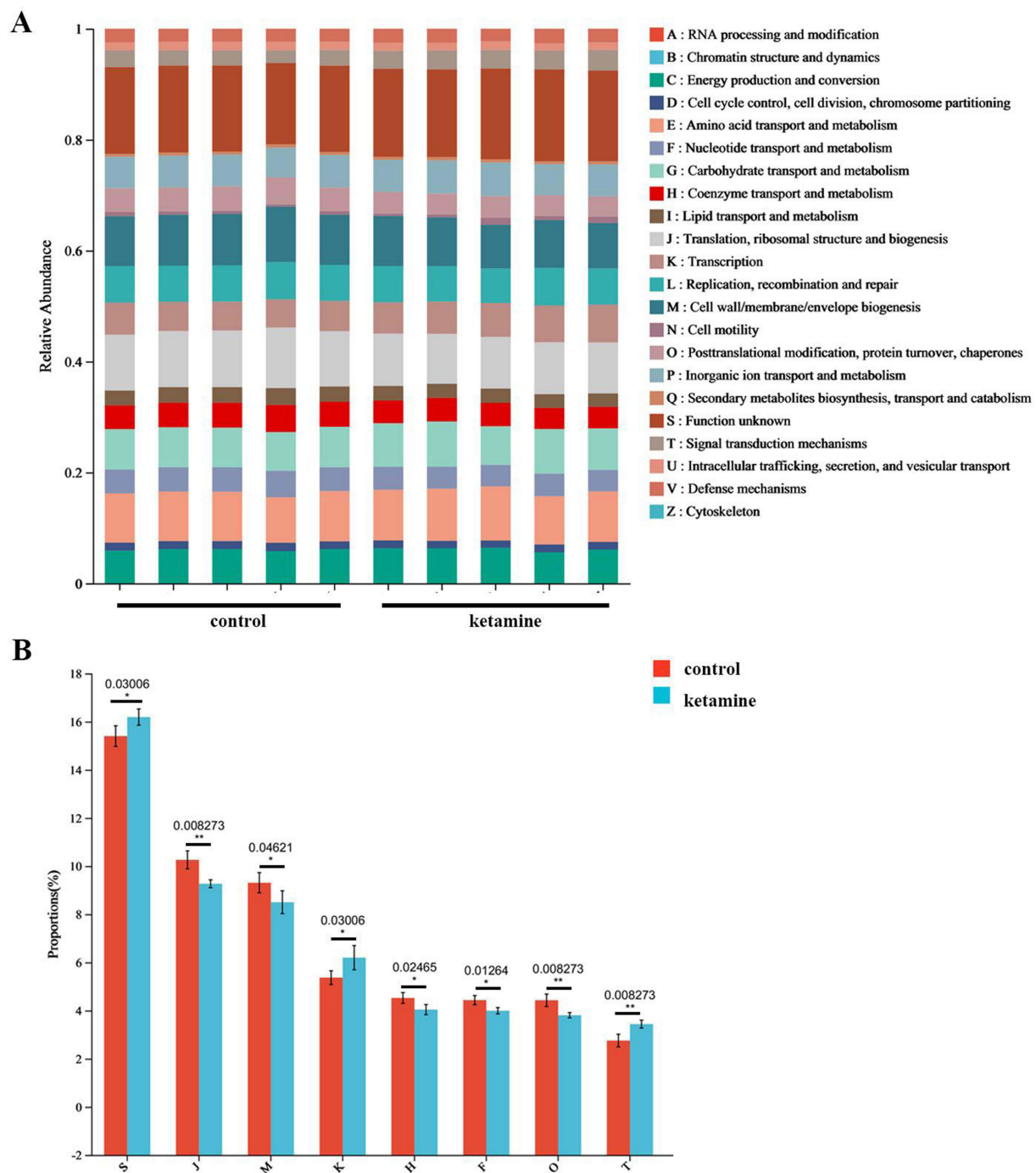
Figure 5 Microbiota function prediction according to COG. (A) The relative abundance of COG function classification in the control and ketamine group ( n = 5 ). (B) The Student's t -test box bloy of COG between two groups. Each bar represents the mean \pm SEM. *P < 0.05 , **P < 0.01 by Student's t -test.
