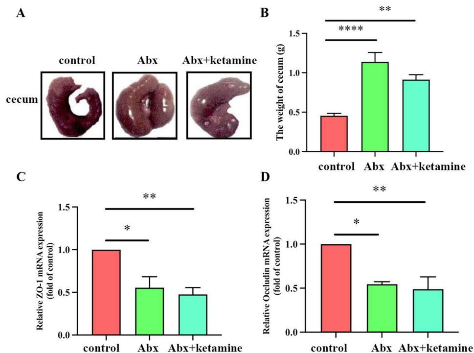
Figure 7 Morphological and barrier disruptions in the intestine induced by gut microbiota depletion. (A) Representative cecal tissues from mice in different groups (n = 8). (B) Analysis of cecum weight. (C) The mRNA expression levels of ZO-1 in colon samples (n = 3). (D) The mRNA expression levels of occludin in colon samples (n = 3). Each bar represents the mean \pm SEM. * P < 0.05 by one-way ANOVA.
