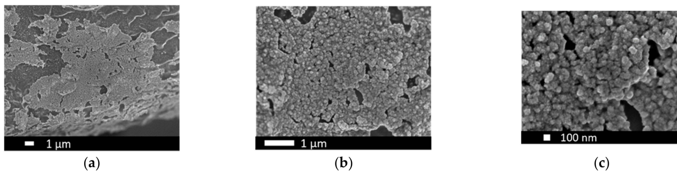
Figure 4. SEM-micrographs of Pt agglomerates obtained via a combined electrochemical deposition method onto Ti-substrate at (a) 5000\times , (b) 20,000\times and (c) 50,000\times magnification.
