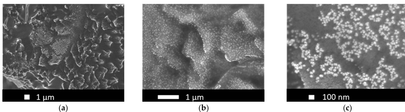
Figure 10. SEM-micrographs of one-step electrodeposited PtIr electrodes at (a) 5000\times , (b) 20,000\times and (c) 50,000\times magnification.
