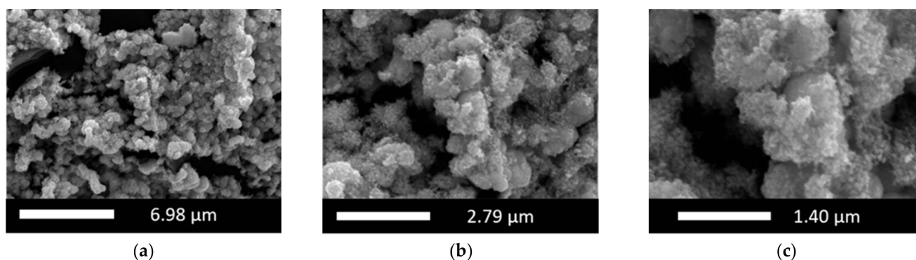
Figure 6. SEM-micrographs of two-step electrodeposited PtIr electrodes at (a) 5000 \times , (b) 20,000 \times and (c) 50,000 \times magnification.
