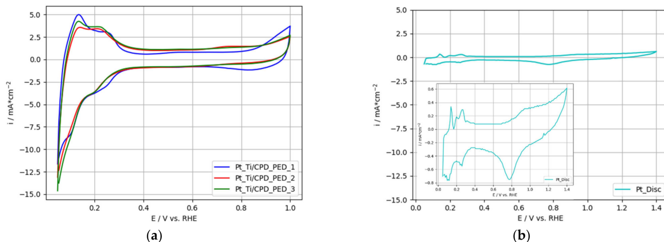
Figure 5. Cyclic voltammograms of (a) Ti-based electrodes with electrochemically deposited Pt, (b) polished, high purity Pt-disc.
