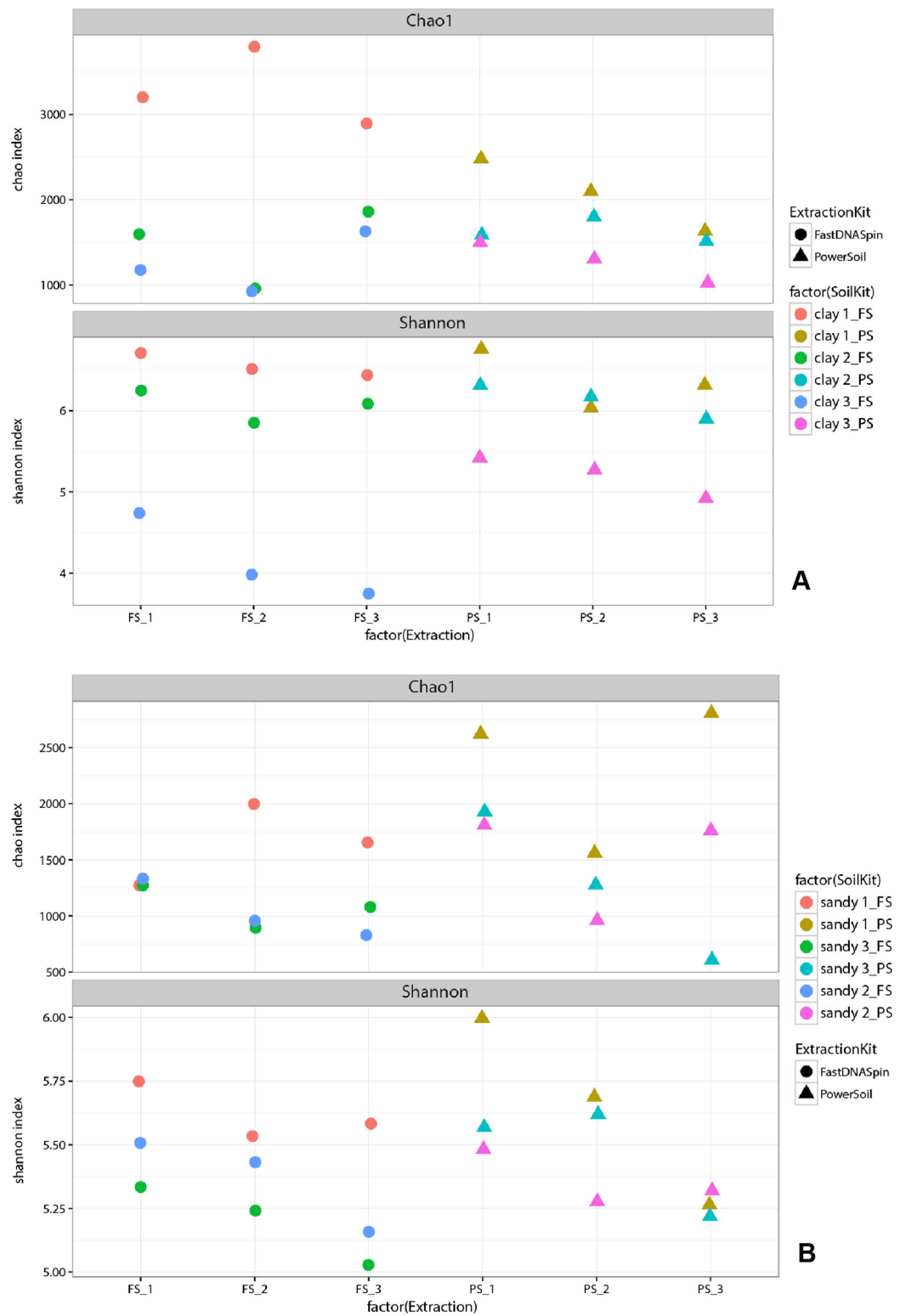
Figure 5 Species richness (Chao1) and diversity (Shannon) of the prokaryotic community in clay (A) and sandy (B) soils.
