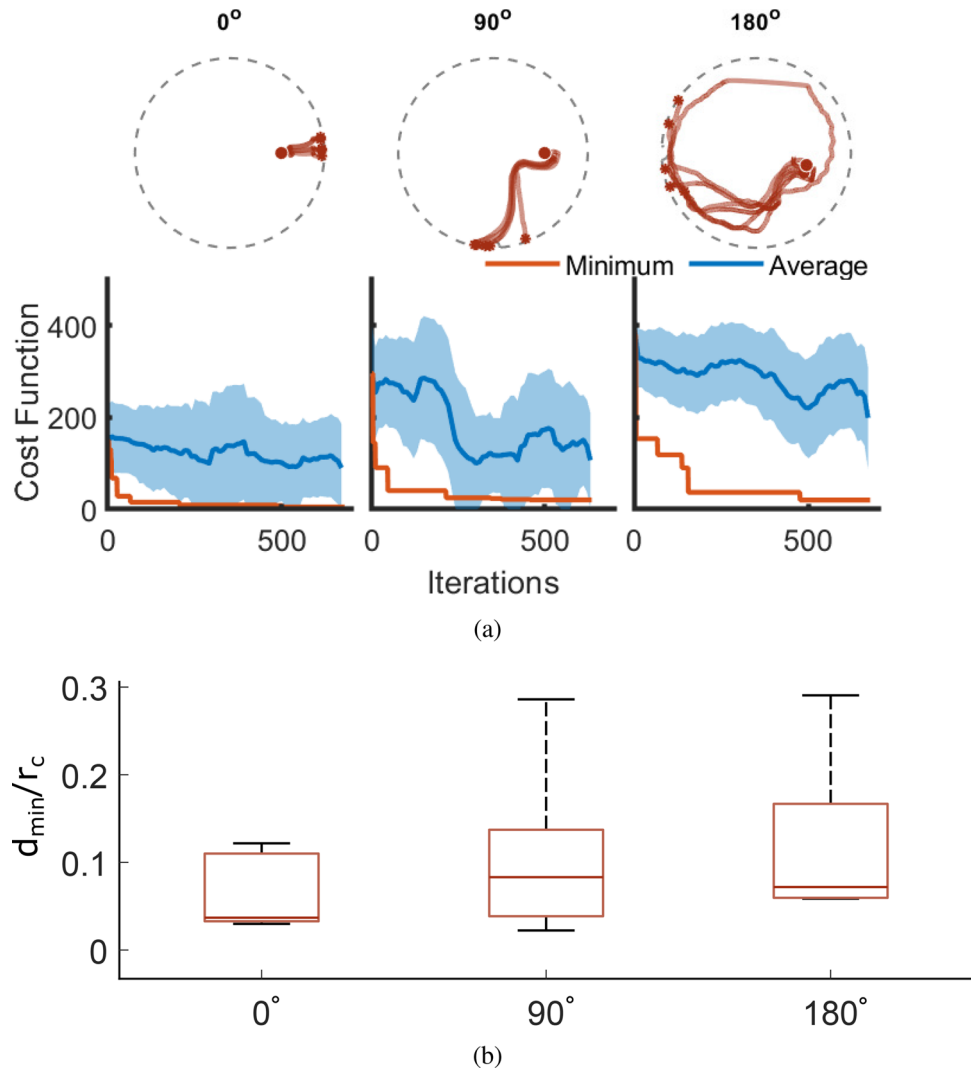
Figure 3. (a) Bayesian optimization results for the 0^\circ , 90^\circ , and 180^\circ open-loop delivery tasks. After 650 iterations, the best set of actions are repeated 5 times and the object's path plotted. (b) Min/max boxplots of the floating object's minimum distance from the target location— d_{min} —during the 5 repetitions, normalized by the container radius r_c .
