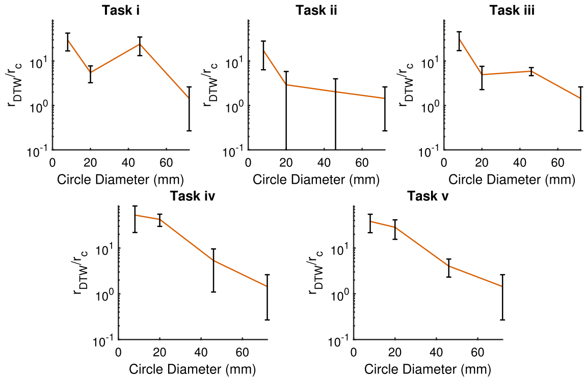
Figure 10. The difference in object trajectories, r_{DTW} , during repetitions of each task for different object diameters. A lower r_{DTW} value indicates a highly repeatable trajectory, representing the minimized local cost measure during dynamic time warping. Values are normalized using the container radius r_c .
