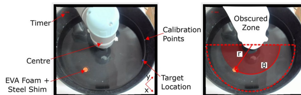
Figure 11. A typical view returned from the camera, indicating the obscured zone, the shaded area in which starting positions are randomized, and the operating semicircle in which target positions are set.
