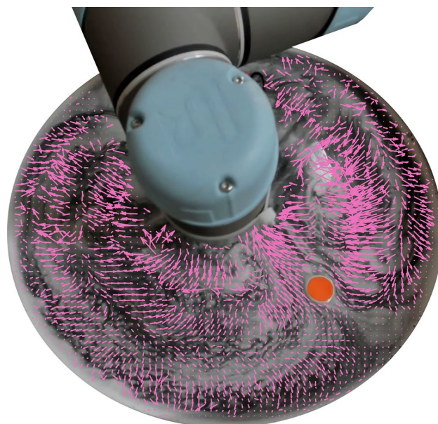
Figure 2. Manipulation of a free-floating object (in orange) by generating surface flows with a robotic arm. The free-floating object is guided across the water by the visualized surface flows.
