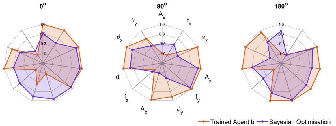
Figure 5. The proposed action spaces for 0°, 90°, and 180° targets. Each of the control parameters is normalized in the range (-1,1).
