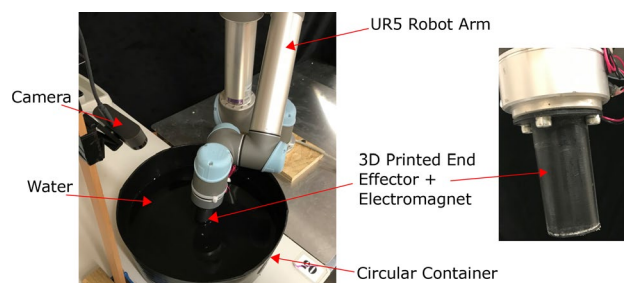
Figure 1. Experimental setup.
