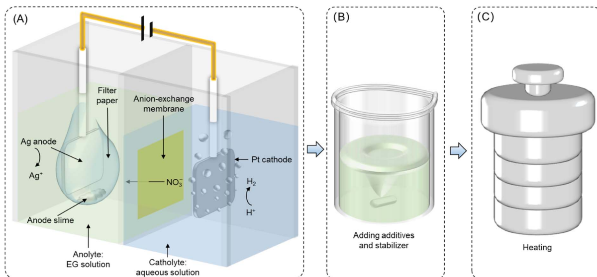
Fig. 2 Procedures and experimental setup of the electrochemical synthesis-polyol reduction method for Ag NP synthesis. (A) Metallic Ag undergoes anodic dissolution in ethylene glycol, while \text{H}_2 evolution occurs at the Pt cathode, \text{Ag}^+ is enriched in anolyte due to the barrier effect of anion-exchange membrane, thereby producing the precursor solution for polyol reduction. (B) The anolyte is added with additives and stabilizer to produce precursor for polyol reduction. (C) The precursor solution undergoes heating to synthesize Ag NPs via polyol reduction.
