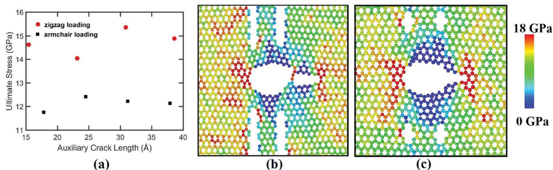
Fig. 5 (a) Variation of ultimate stress with the variation of the length of the auxiliary cracks ( r = 28.4 Å and \theta = 70.3^\circ for armchair and r = 43.6 Å and \theta = 76.7^\circ for zigzag loading cases). Failure initiation for the cases of (b) largest and (c) smallest auxiliary crack length. Because of the high plasticity, failure occurs ahead of the main crack tip for the largest auxiliary crack length.
