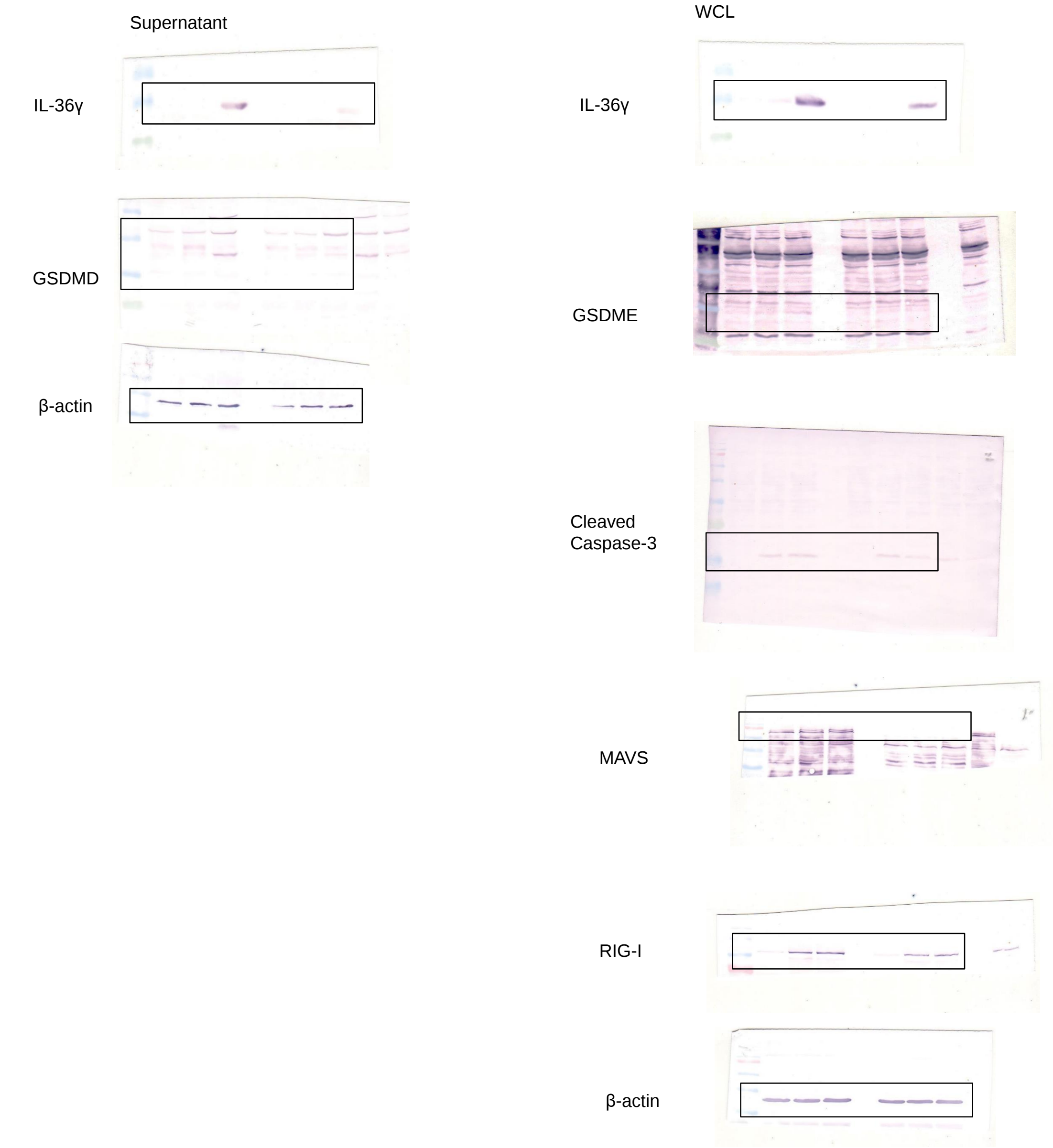
Figure 5 D
