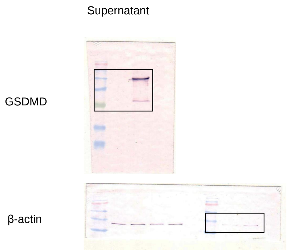
Figure 1 G
