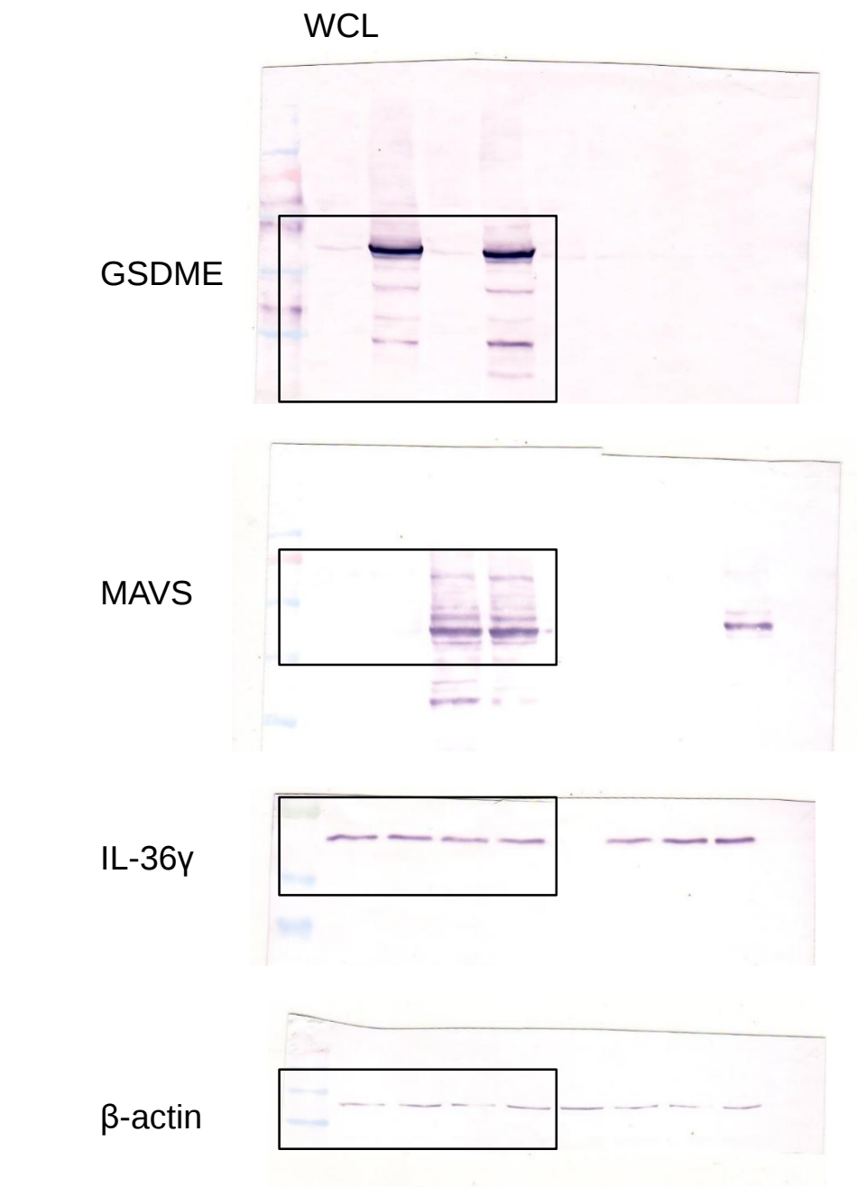
Figure 6 F
