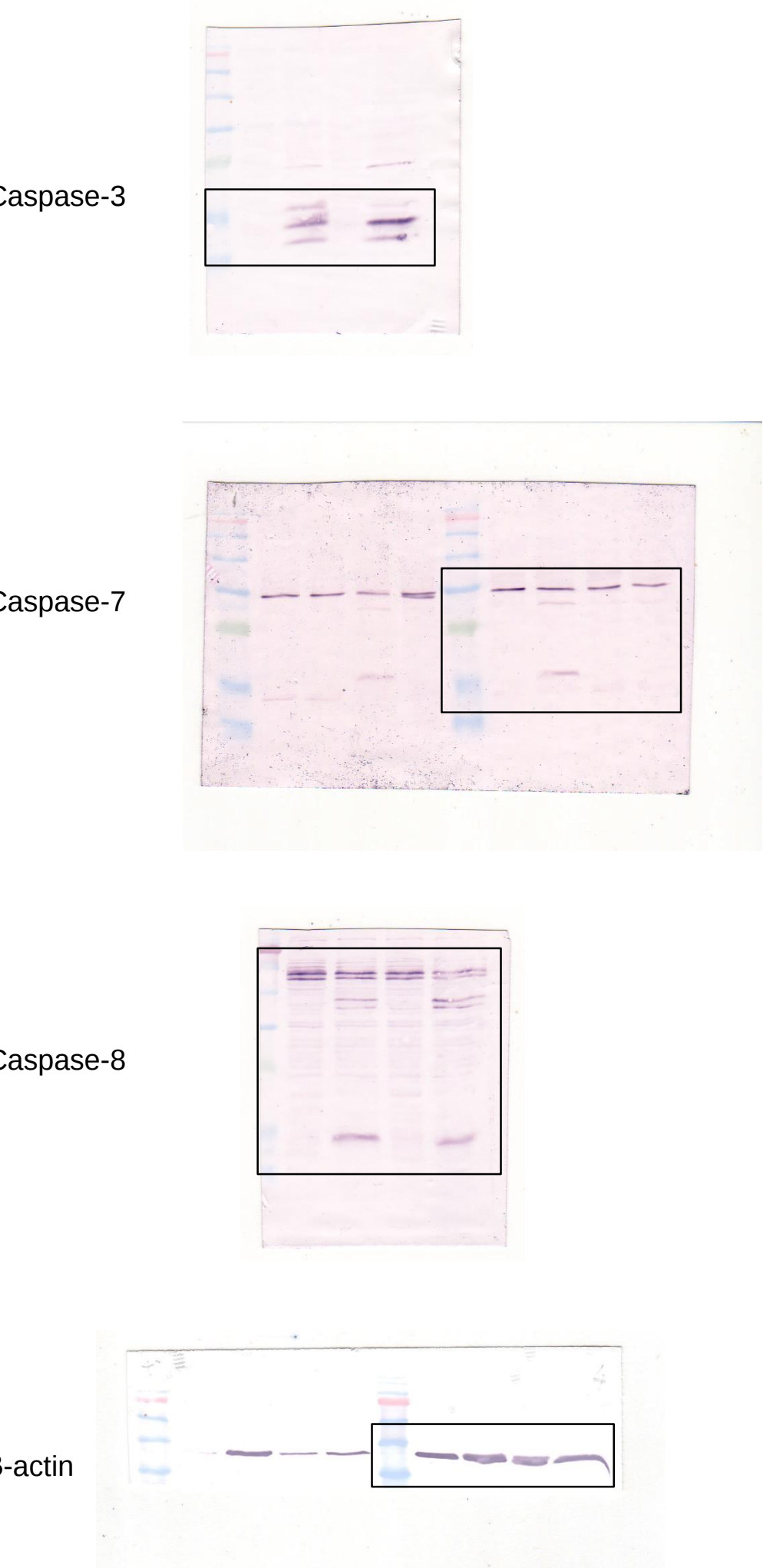
Figure 1 F
