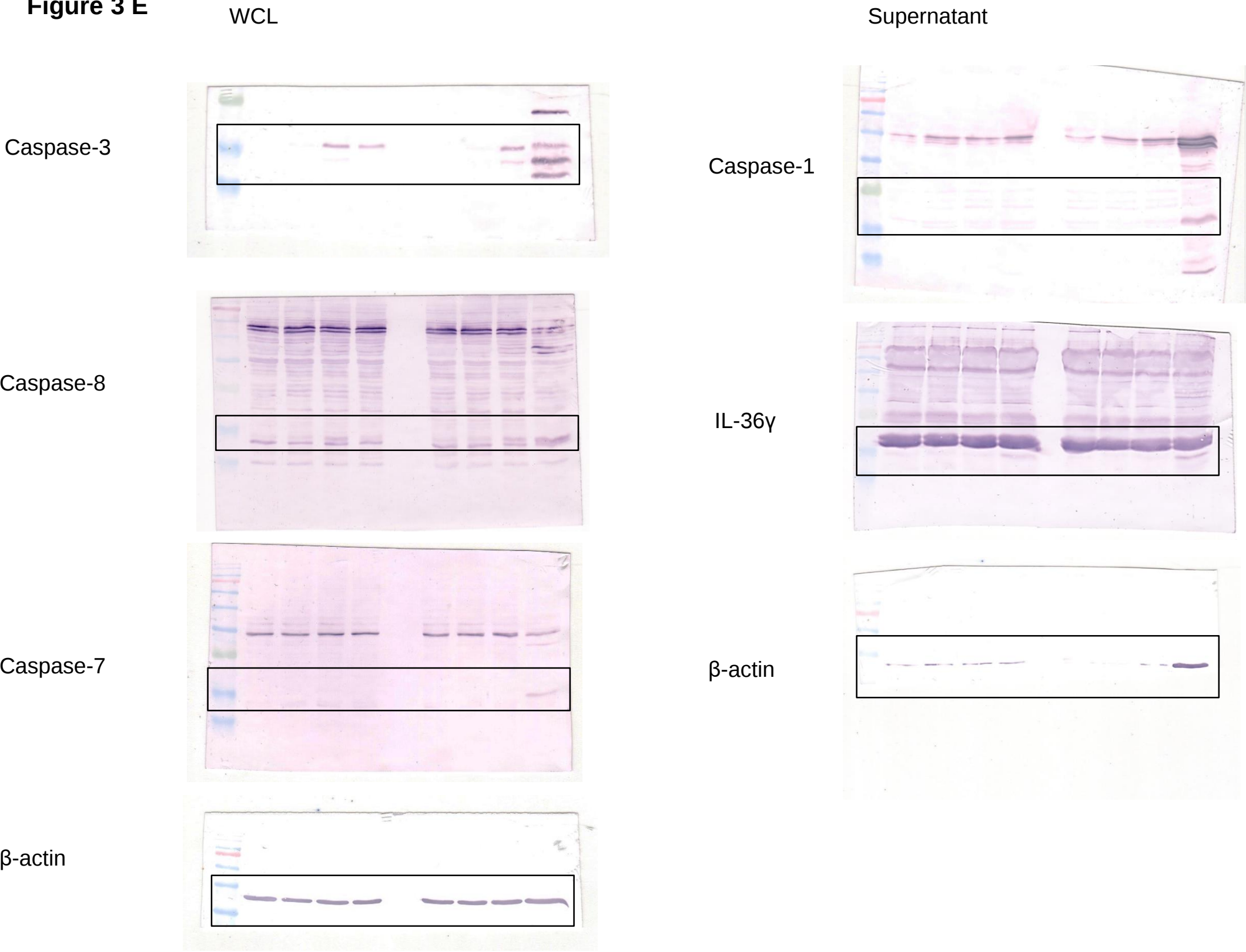
Figure 3 E
