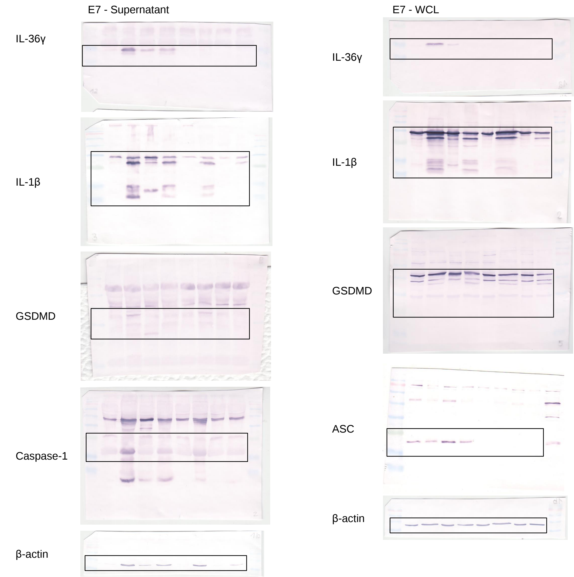
Figure 1 F
