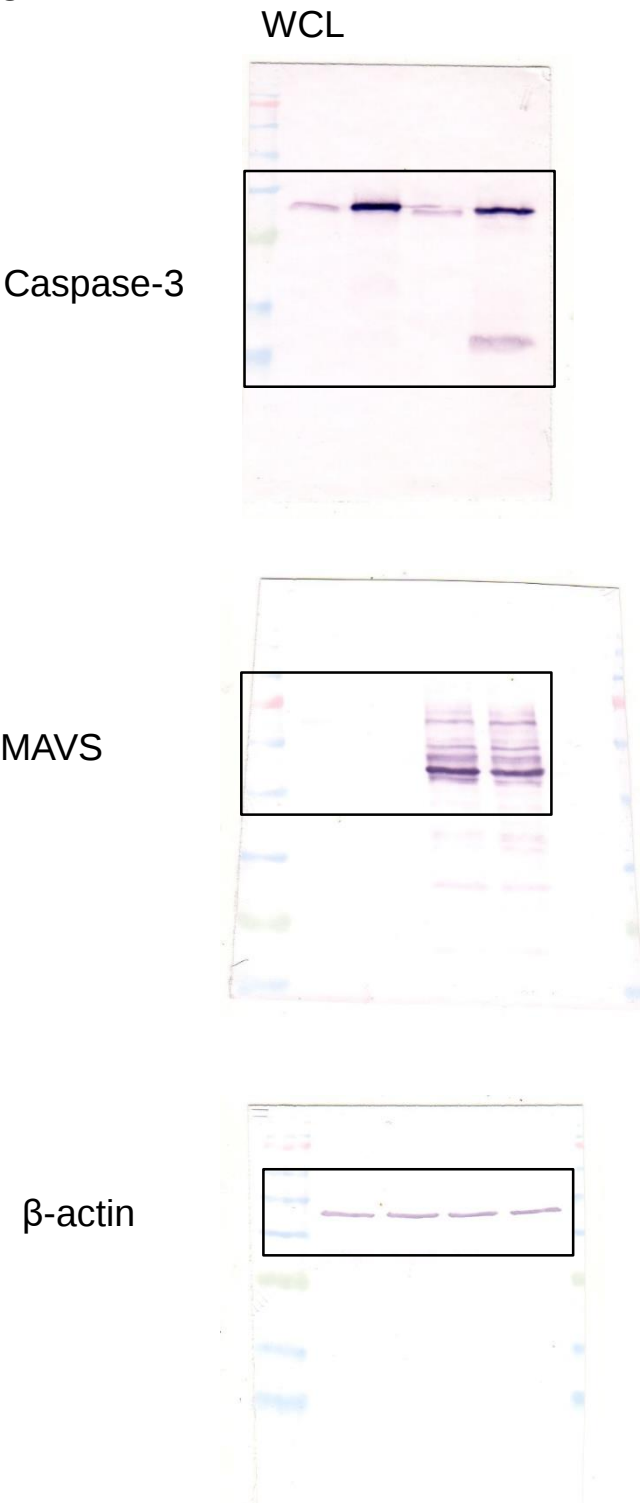
Figure 5 F
