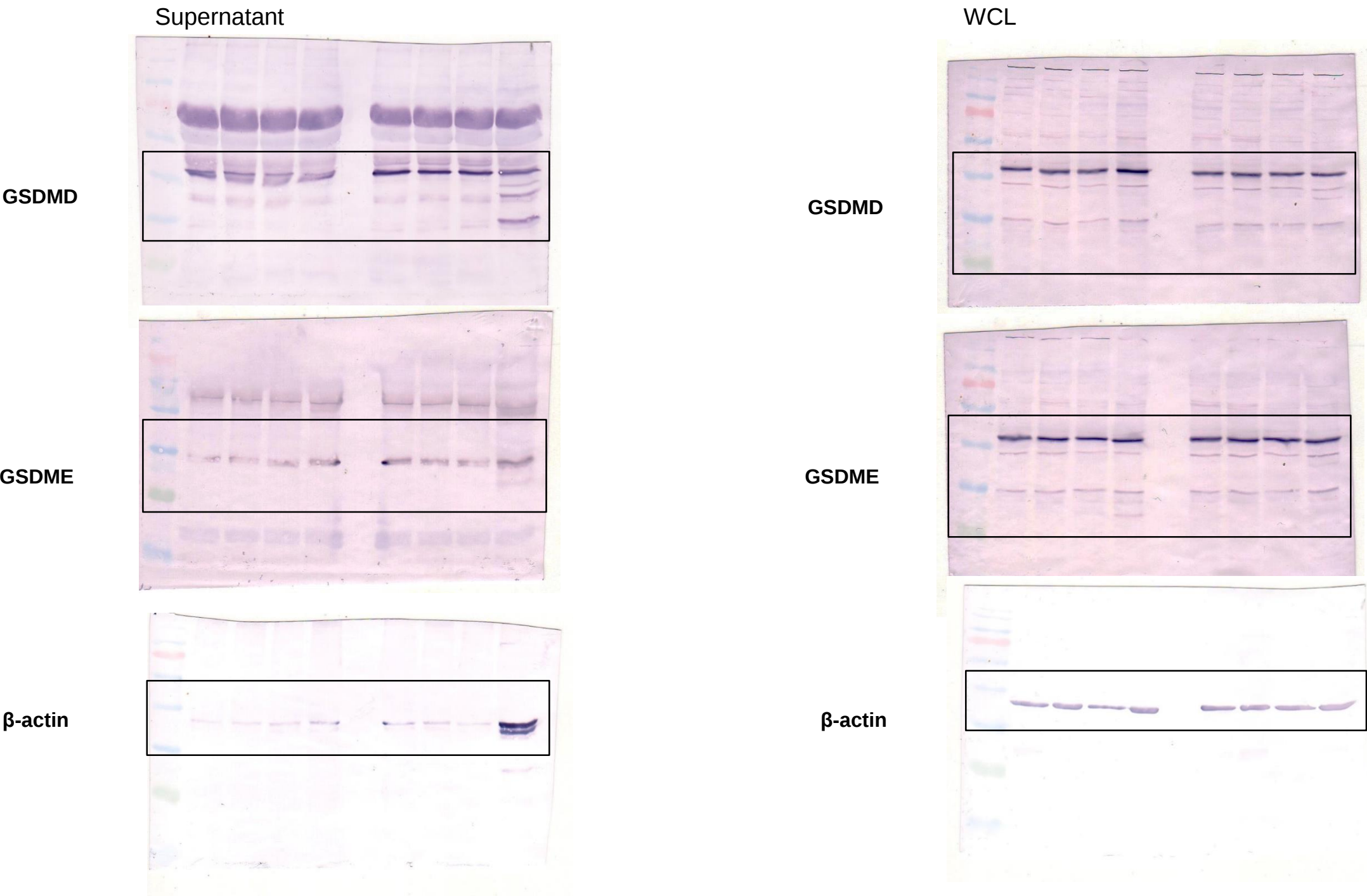
Figure 3 F
