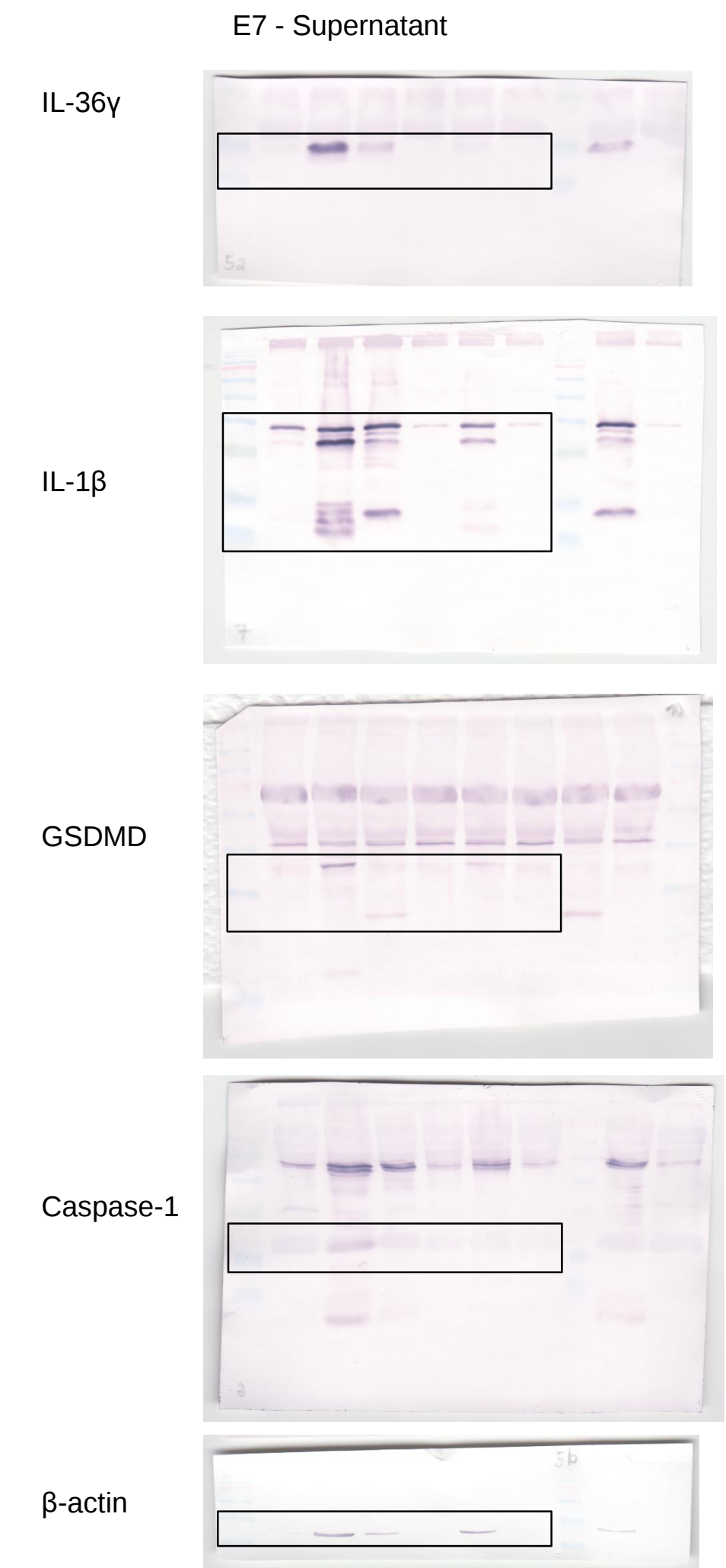
Figure 2 D
