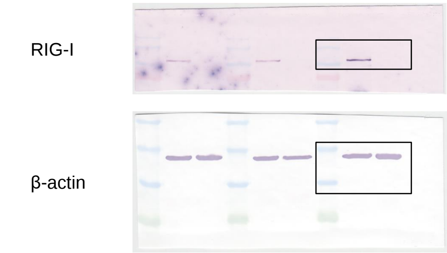
Figure 6 D
