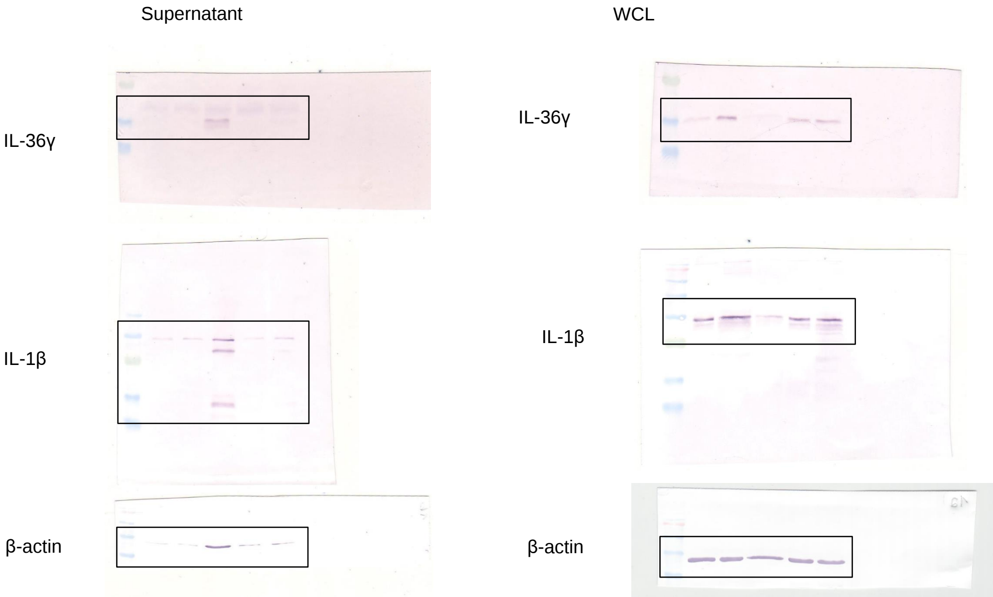
Figure 1 A
