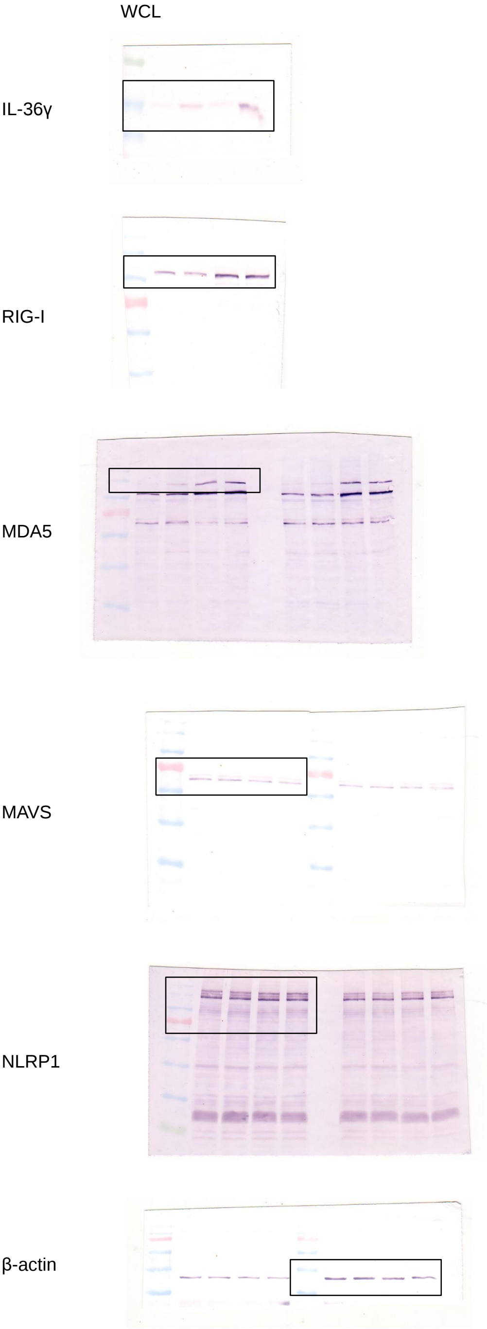
Figure 4 C
