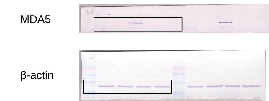
Figure 6 E
