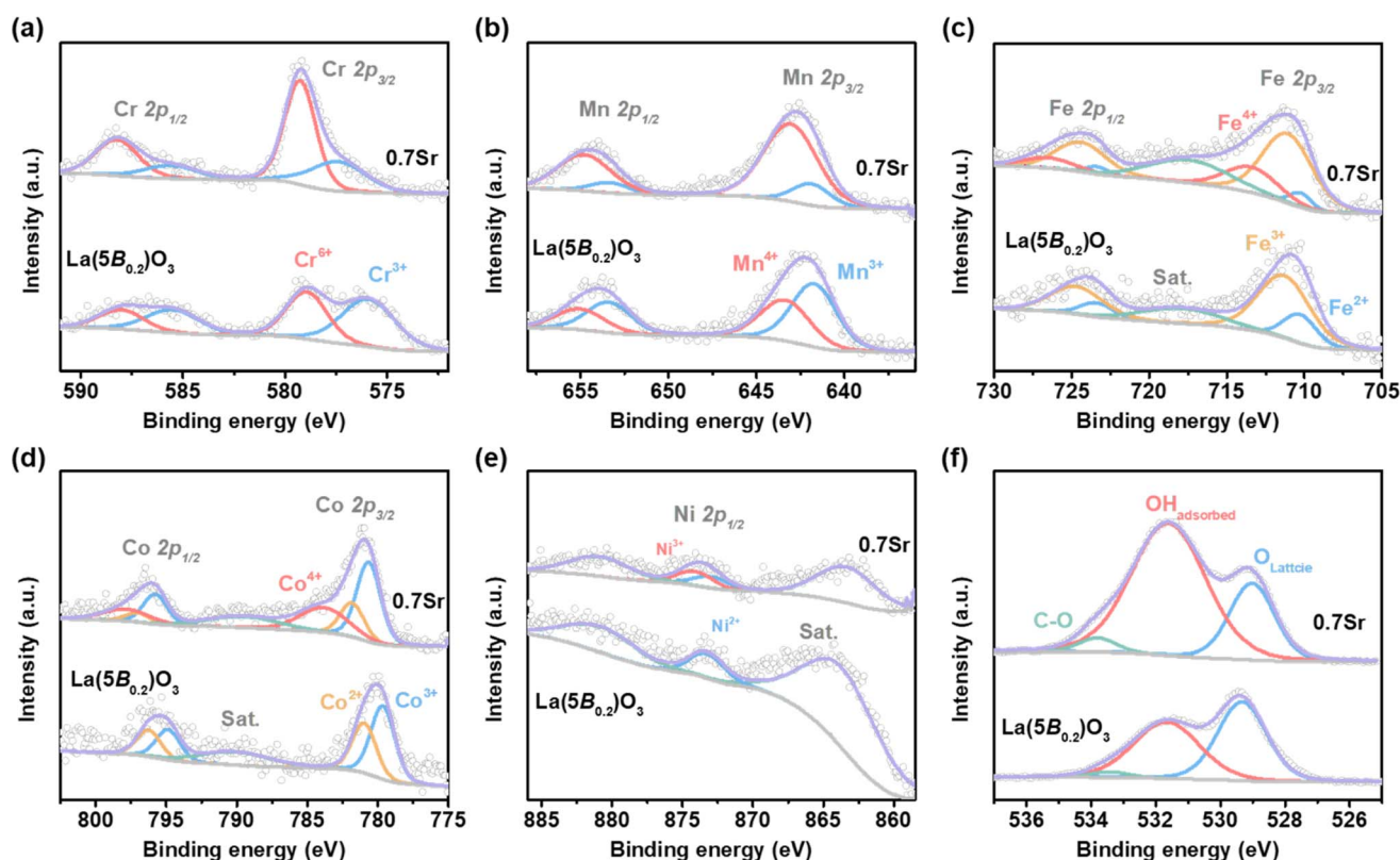
Fig. 6 XPS spectra for La(5B 0.2 )O 3 and 0.7Sr. (a) Cr 2p, (b) Mn 2p, (c) Fe 2p, (d) Co 2p, (e) Ni 2p and (f) O 1s.
