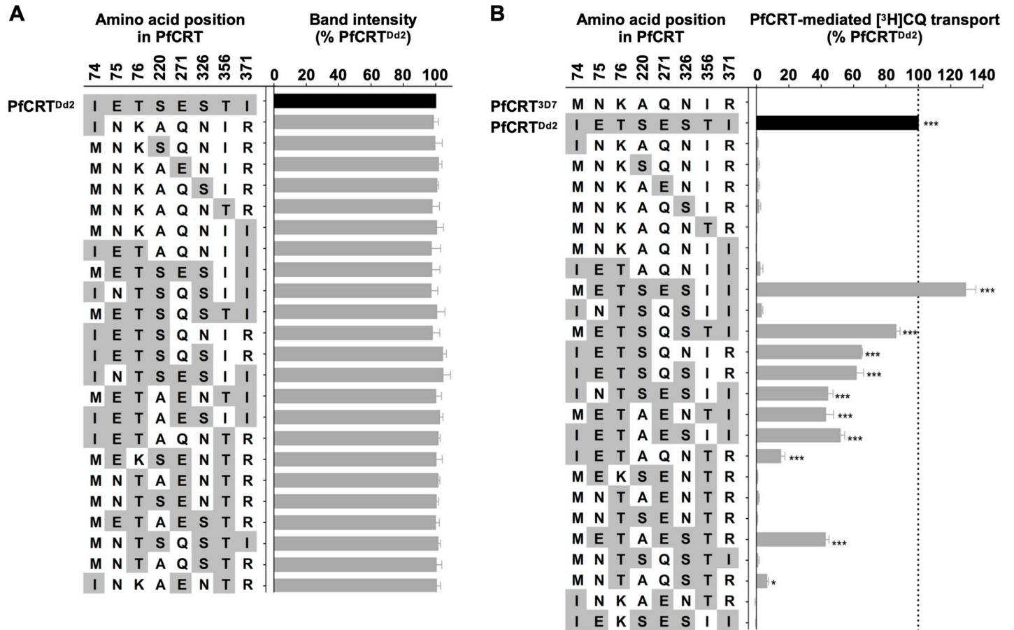
Fig 3. Experimental characterization of the 24 combinatorial variants. (A) The level of PfCRT protein in the oocyte membrane was semi-quantified using an established western blot approach [24]. The analysis included PfCRT Dd2 as a positive control, to which the other band intensity values were normalized. Sample loading and transfer of the proteins were evaluated by total protein staining of the nitrocellulose membrane. The data are the mean + SEM of at least three independent experiments (performed using oocytes from different frogs), within which measurements were averaged from two independent replicates. There were no significant differences in expression levels between the 24 variants of PfCRT ( P > 0.05 ; one-way ANOVA). That is, all of the PfCRT variants were present at similar levels in the oocyte membrane and any differences in CQ transport activity between these proteins are thus attributable to the mutations they carry, rather than differences in expression levels. (B) [ 3 H]CQ transport was measured at pH 5.5 and in the presence of 15 \mu M unlabeled CQ. The direction of CQ transport in oocytes is equivalent to the direction of CQ transport in the malaria parasite (S1 Fig). The PfCRT-mediated component of CQ transport was calculated by subtracting the level of CQ accumulation detected in non-expressing oocytes (the negative control) from that measured in oocytes expressing a PfCRT variant. The rate of PfCRT-mediated transport was then expressed relative to that measured in oocytes expressing PfCRT Dd2 (the positive control). The data are the mean + SEM of at least three independent experiments (performed using oocytes from different frogs), within which measurements were made from 10 oocytes per treatment. The asterisks denote a significant difference in CQ transport between oocytes expressing PfCRT 3D7 (the wild-type isoform) and oocytes expressing another variant of PfCRT: *, P < 0.05 ; ***, P < 0.001 (one-way ANOVA or Student's t -test). In both panels, the data for IEKSESII (i.e. the '106/1' isoform of PfCRT) was taken from Richards et al., 2016 [75]. The presence at the oocyte plasma membrane of the variants of PfCRT lacking significant CQ transport activity was confirmed via immunofluorescence assay (S2 Fig, S3 Fig).
