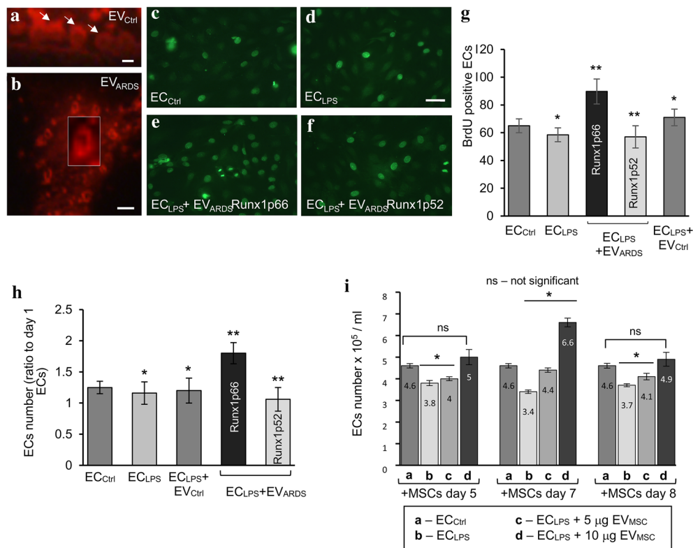
Fig. 5 EV ARDS Alk5Runx1p66 increase proliferation of LPS-treated ECs. Biotin/neutrAvidin–Alexa Fluor 594 labeling of EVs isolated from a human healthy donor (a, EV Ctrl ) and an ARDS subject (b, inset; EV ARDS ). Arrows in a indicate several donut-shaped EV Ctrl . Bars: 1 μm (a, and b inset), 2 μm (b). n = 3. BrdU labeling of EC Ctrl (c), EC LPS (d) and EC LPS exposed to EV ARDS Alk5Runx1p66 isolated from the blood of a long-term ARDS survivor (e) and EC LPS exposed to EV ARDS Alk5Runx1p52 isolated from the blood of a non-surviving ARDS patient (f). A dose of 1.6 \times 10^3 EV ARDS /1 ml growth medium was used for the micrographs shown. Bars: 50 μm (c–f). g Quantification of BrdU-positive cells. The results are expressed as BrdU-positive ECs/high power field (50 power field images/experimental condition). Data are representative of three different experiments and were normalized per total number of cells counted. Values are shown as mean ± SEM. n = 3; *p < 0.05; **p < 0.01. h MTT assay and cell counting of EC Ctrl and EC LPS exposed for 3 days to EV Ctrl and EV ARDS , as above (ratio 2:1 EV ARDS :EV Ctrl ). Data are normalized to day 1 EC Ctrl . Values are shown as mean ± SEM. n = 3; *p < 0.05; **p < 0.01. i EC Ctrl (a bars), EC LPS (b bars), EC LPS + 5 μg EV MSC (c bars) and EC LPS + 10 μg EV MSC (d bars) were counted 3 days post-EV MSC exposure. Briefly, EV MSC released by 3 \times 10^6 MSCs, at day 5, day 7 and day 8, were resuspended in 50 μl sterile PBS; 1 dose of 10 μg/ml protein was found efficient in inducing proliferation of EC LPS . All data labels are included for each bar. Values are shown as mean ± SEM. n = 3 experiments (triplicate wells each); *p < 0.01 vs. EC Ctrl
