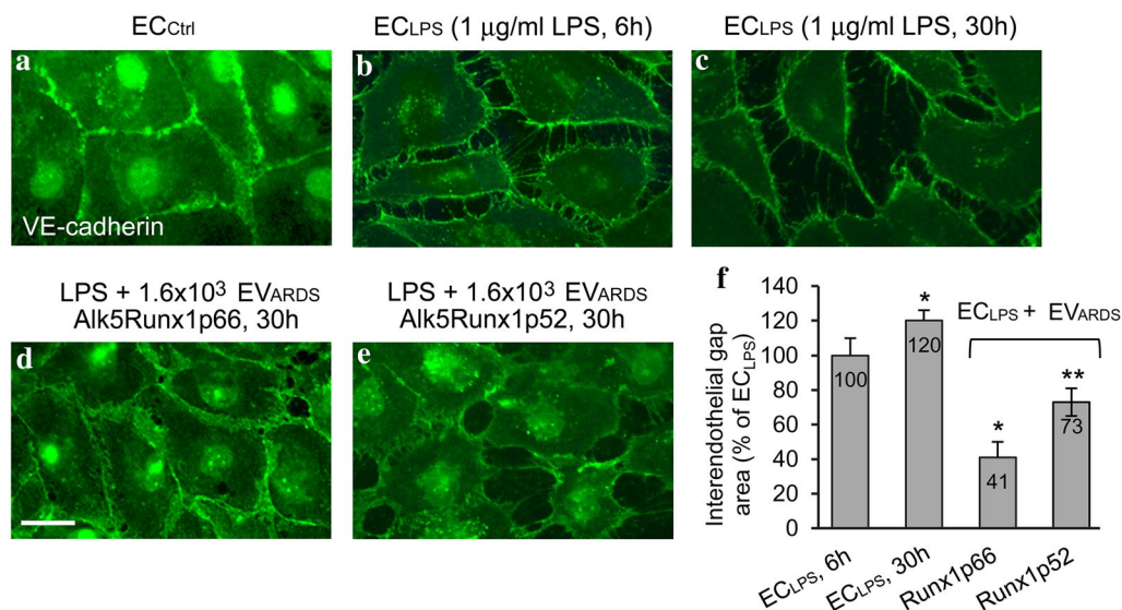
Fig. 6 EV ARDS Alk5Runx1p66 improve the interendothelial junctional integrity of LPS-treated ECs. Representative VE-cadherin/Alexa Fluor 488 staining of EC Ctrl ( a ), ECs treated with 1 \mu g/ml LPS (EC LPS ) for 6 h ( b ) and 30 h ( c ); EC LPS (6 h) were treated for 30 h with either ( d ) 1.6 \times 10^3 EV ARDS Runx1p66/1 ml growth media or ( e ) 1.6 \times 10^3 EV ARDS Runx1p52/1 ml growth media (non-surviving ARDS patient). Bars: 15 \mu m ( a–e ). f Morphometric analysis of the interendothelial gap area. All data labels are included for each bar. n = 3 EVs preparations/experimental condition, in three independent experiments; * p < 0.01 ; ** p < 0.05
