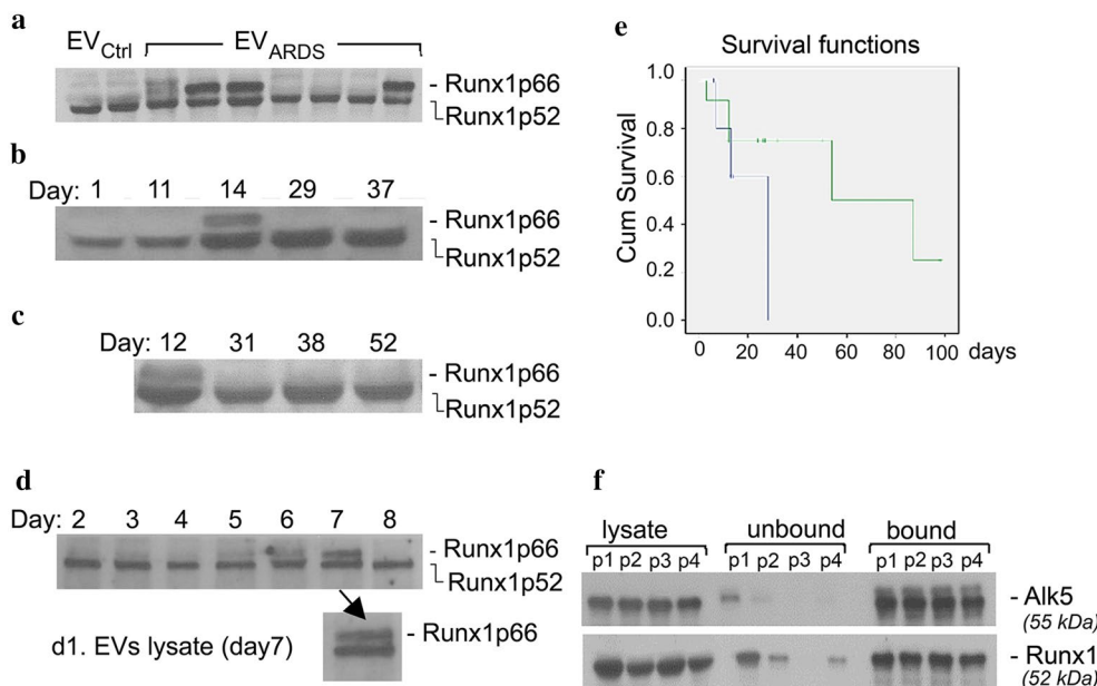
Fig. 4 Runx1p66 protein expression is short-lived and provides a survival advantage. a Representative Western blot of Runx1 protein expression in seven EV ARDS and two EV Ctrl preparations. Normalization was achieved to the volume of blood used (typically 1.5 ml) for EVs isolation. b Time course analysis of Runx1 in EV ARDS of a long-term ARDS survivor (S6) and panel c , a non-surviving ARDS patient (S12). Expression of Runx1p52 gradually increases from day 1 to day 37 in ICU in the EV ARDS of long-term survivor. Even if the number of blood samples available for later time points assessed was lower due to death of some patients, the time course analysis data are representative for at least three long-term survivors and three non-surviving ARDS patients. d Western blot of Runx1 expression in lysates of cultured human bone marrow-derived MSCs (d2–d8) as well as in lysates of the EV MSC released at d7 (d1). 30 µg protein/lane; n = 3. e The Kaplan–Meier statistic shows the improved survival for the EV ARDS Alk5Runx1p66 patients. Out of 33 ARDS patients included in the study, only 29 patients (multiple samples) were used to investigate the Runx1 isoform content and the Runxp66/p52 ratio. f Four EV ARDS preparations (p1–p4; isolated from 1.8 ml of blood) were labeled with a biotinylated Alk5 rat Ab followed by streptavidin-conjugated magnetic beads. An isotype matched IgG for Alk5 was used as control. Aliquots of EV ARDS lysates, unbound and bound fractions were analyzed by SDS PAGE and Western blot with Alk5 and Runx1 Abs. EV ARDS are immunoreactive to Runx1p52 isoform only as the blood samples used belong to either non-surviving ARDS subjects or to surviving ARDS subjects, but collected in week 1 of ICU stay, when the EV ARDS do not show Runx1p66 immunoreactivity. n = 9 different ARDS patients; Three independent experiments were performed
