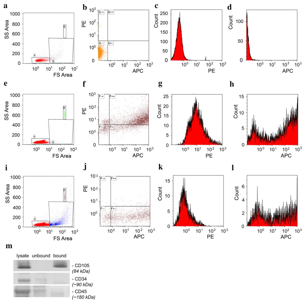
Fig. 3 EV ARDS Alk5 sub-population is derived from the MSCs. Unstained EVs were used as controls to determine fluorescence background as well as for gating purposes. a Representative forward and side scatter plot for unstained EVs. Background fluorescence in the PE and APC channels for the unstained samples shown as dot plot ( b ) and individual histograms ( c, d ). Similar, representative plot of EVs stained with Alk5-APC/CD105-PE Abs ( f ) to analyze the co-expression of these markers on the EV ARDS ( e , Gate D), together with the individual histograms for CD105-PE ( g ) and Alk5-APC ( h ). Representative plot of EVs stained with Alk5-APC/CD73-PE Abs ( j ) to analyze the co-expression of these markers on the EV ARDS ( i , Gate D), along with the histograms for CD73-PE ( k ) and Alk5-APC ( l ) are also shown. n = 9 EV ARDS and 5 EV Ctrl isolates. m Representative immunoprecipitation of CD105 + EV ARDS Alk5 via biotin-conjugated CD105 Ab and streptavidin magnetic beads incubation. Lysates of EV ARDS , bound and unbound EV ARDS fractions were analyzed by SDS PAGE and WB. No immunoreactivity to CD45 and CD34 is detected. n = 6 EVs isolates/experimental condition, in three independent experiments
