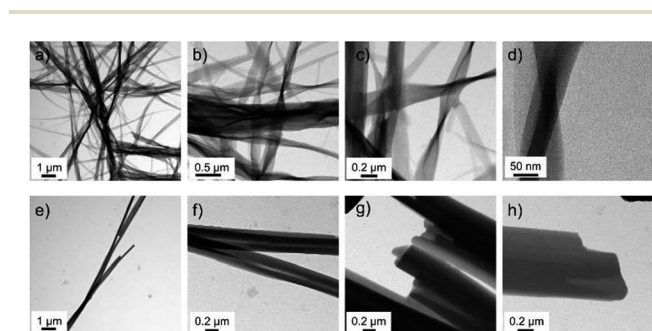
Fig. 5 Transmission electron micrographs of nanowires obtained from dried isooctane solutions of (a–d) CuL8 and (e and f) CuL16.
