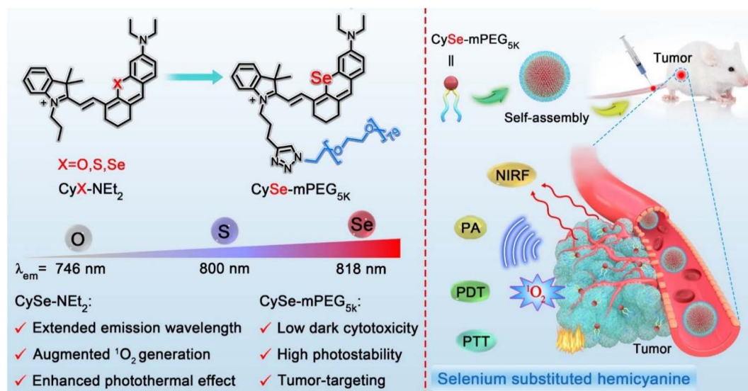
Scheme 1 Chemical structures of CyX- \text{NET}_2 (X = O, S, Se) and CySe-mPEG 5K , and the schematic illustration of tumor targeting imaging-guided phototherapy.
