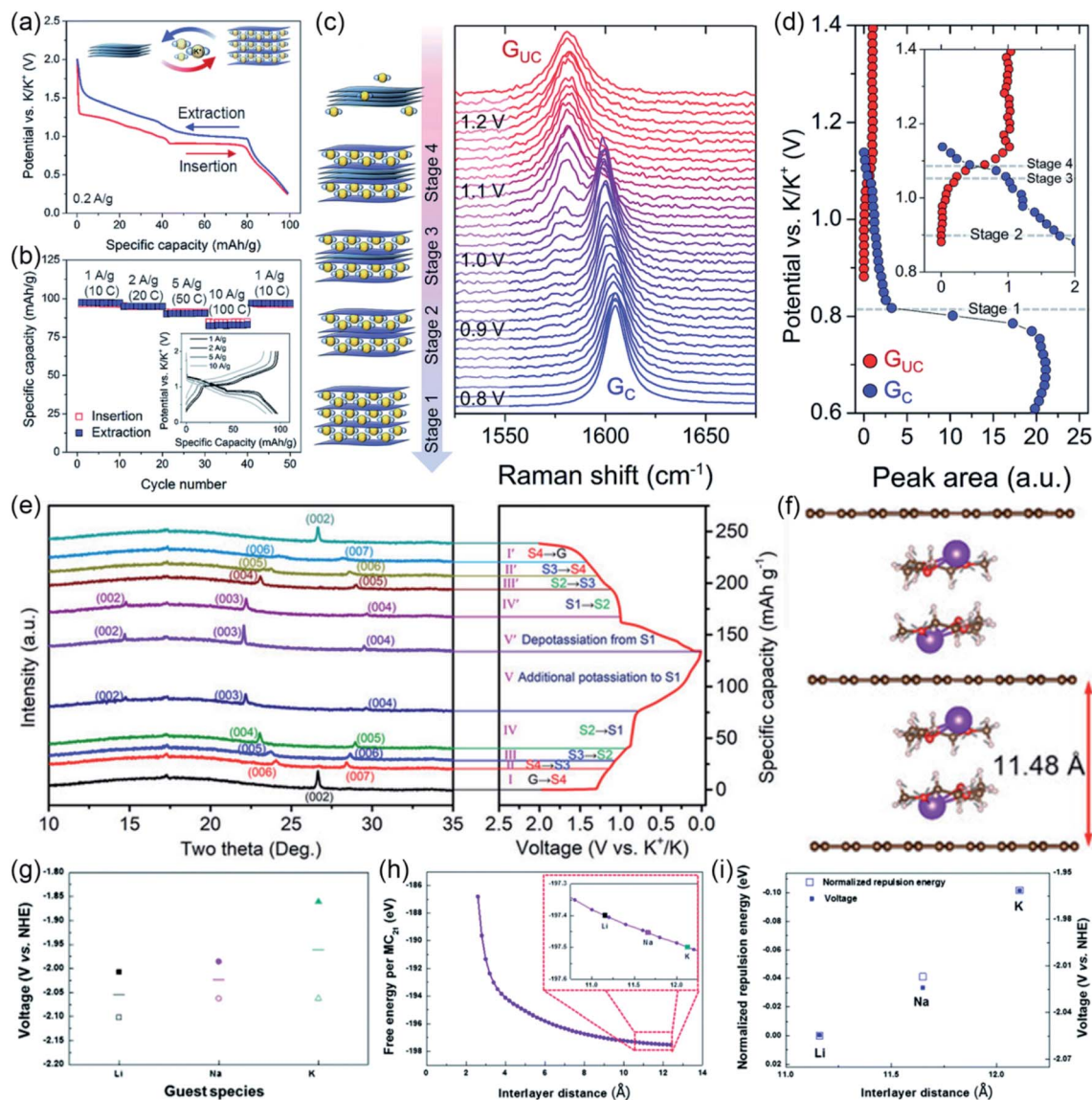
Fig. 7 Ion-solvent co-intercalation species in PIBs. (a) Charge/discharge curves and (b) rate performance (inset: corresponding charge/discharge curves) of MLG foam in ether-based electrolyte. (c) In situ Raman spectrum of MLG foam. (d) The relative peak areas of the two G peaks. (a–d) Reproduced with permission. 38 Copyright 2016, Royal Society of Chemistry. (e) The partial XRD patterns of characteristic stages of the GICs and the corresponding charge/discharge curves. (Note: S1, stage 1; S2, stage 2; S3, stage 3; S4, stage 4; G, graphite.) (f) The structure of two [K-DEGDME] + complexes intercalated in graphite (red, gray, white and purple balls represent O, C, H and K atoms, respectively). (e and f) Reproduced with permission. 77 Copyright 2020, Wiley-VCH. (g) The average voltage of graphite electrode in different battery systems (line: average voltage, filled symbols: charge voltage, empty symbols: discharge voltage). (h) Free energy of the negatively charged graphite framework (one charge injected in 21 C atom) as a function of interlayer distance (inset: magnification of the red square). (i) Voltage and normalized repulsion energy as a function of interlayer distance (filled squares: voltage, open squares: normalized repulsion energy). (g–i) Reproduced with permission. 78 Copyright 2016, Royal Society of Chemistry.
