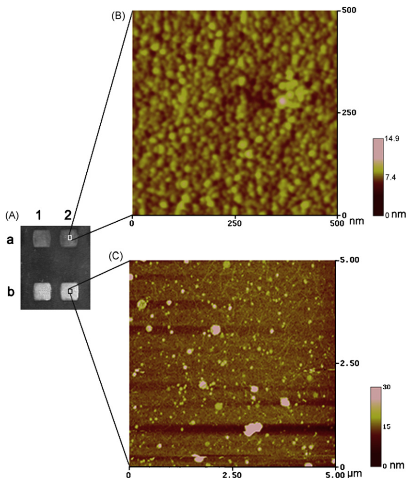
Fig. 5. The result of phage detection of antibody GP3 and phage M13KO7 by using BIE and AFM height images, respectively. (A) The result of BIE: antibody GP3 was immobilized and formed four areas “a1, a2, b1, b2”, among which “b1, b2” were adopted to detect phage sample. After BIE detection, the chip is submitted to AFM for scanning: (B) AFM image of scanning under 500 nm on the area containing antibody GP3; (C) AFM image of scanning under 5 μm on the area dedicated for phage detection.
