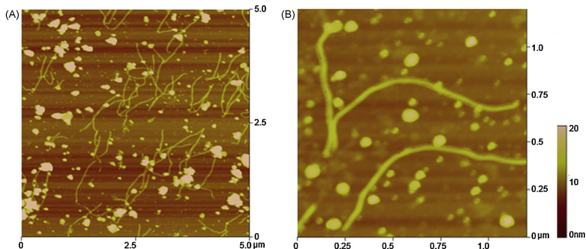
Fig. 4. AFM height images of phage M13KO7 on the mica surface. Image “A” was scanned under 5 \mu\text{m} and 0.8846 Hz and “B” was scanned under 1.2 \mu\text{m} and 1.209 Hz.
