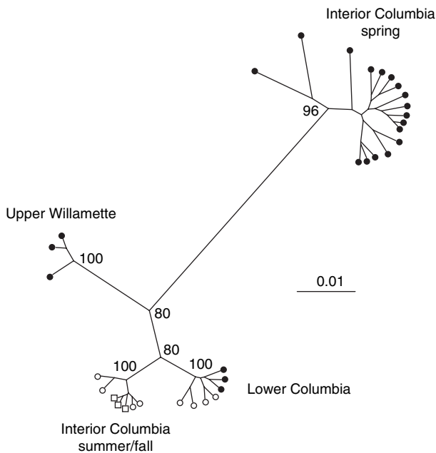
Figure 6 Life history variation mapped onto a tree depicting population genetic structure of Columbia River Chinook salmon. Each population is represented by a symbol indicating the peak run timing (time of entry of adults into fresh water on their spawning migration): solid circle = spring; open square = summer; open circle = fall. Support for the four major genetic lineages (two from the Interior Columbia River, east of the Cascades, and two from west of the Cascades) is indicated by numbers at nodes (percent of 1000 bootstrap replicates having the identical tree topology). Modified from Waples et al. (2004).
