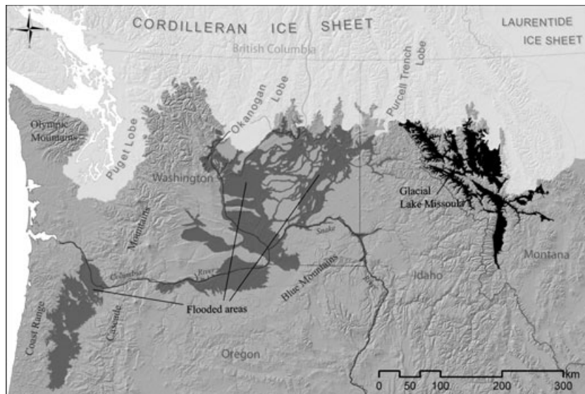
Figure 3 Map of the Pacific Northwest showing areas flooded in the late Pleistocene by periodic breaching of the ice dam that blocked outflow of the Clark Fork River (a tributary to the Columbia River) and created Glacial Lake Missoula.
