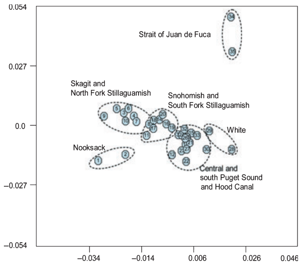
Figure 5 Multidimensional scaling plot of pair-wise genetic distances among populations of Chinook salmon in Puget Sound. Modified from Ruckelshaus et al. 2006.
