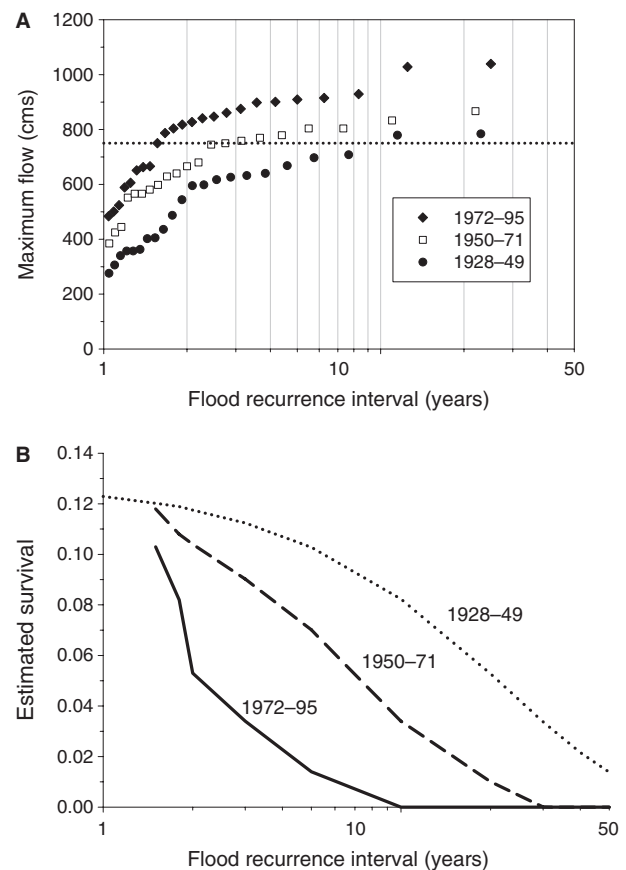
Figure 4 (A) Change over time in the magnitude of flood events in the North Fork Stillaguamish River, Washington, USA. Raw data are largest annual peak flows from a US Geological Survey stream gauge ( http://waterdata.usgs.gov/wa/nwis/uv?station=12167000 ). To calculate the flood recurrence interval, we fit the annual maximum peak discharge data to a log-Pearson Type III distribution using a method of moments approach (US Water Resources Council 1981, Sumioka et al. 1998). (B) Estimates of egg-to-fry survival associated with flood events depicted in the top graph based on the model developed by Seiler et al. (2002) for Chinook salmon from the nearby Skagit River.
