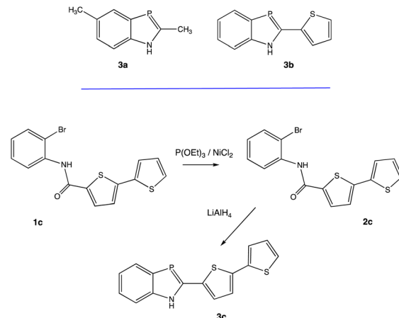
Scheme 1 1 H -1,3-benzazaphospholes 3a and 3b (top), preparation of 3c (bottom).
