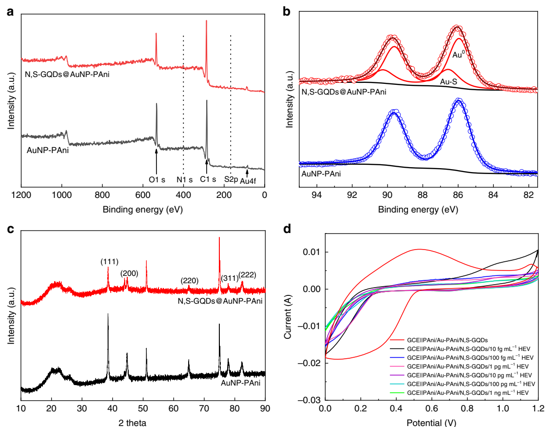
Fig. 3 Characterizations of N,S-GQDs@AuNP-PAni nanocomposites: a survey spectrum of XPS, b deconvoluted Au 4f spectra, c XRD of N,S-GQDs@AuNP-PAni nanocomposites before and after attachment of N,S-GQDs, and d cyclic voltammetry (CV) of the Ab-N,S-GQDs@AuNP-PAni/PAni||GCE sensor electrode before and after the addition of different virus concentrations
