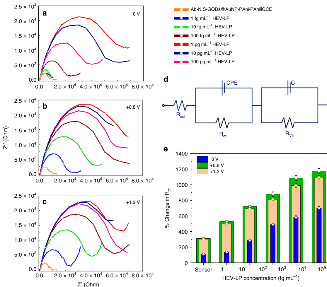
Fig. 4 Electrochemical impedimetric performances over electric pulse on the sensor electrode with different virus concentration: EIS of Ab-N,S-GQDs@AuNP-PAni/PAni|GCE sensor electrode before and after incubation with 1 fg mL -1 to 100 pg mL -1 of HEV-LP with external pulses of a 0 V, b +0.8 V, and c +1.2 V. Circuit diagram of the proposed sensor ( d ) and comparative diagram of percentage change in R_{ct} values in three pulse conditions ( e ). Error bars represent the standard deviation of triple measurements
