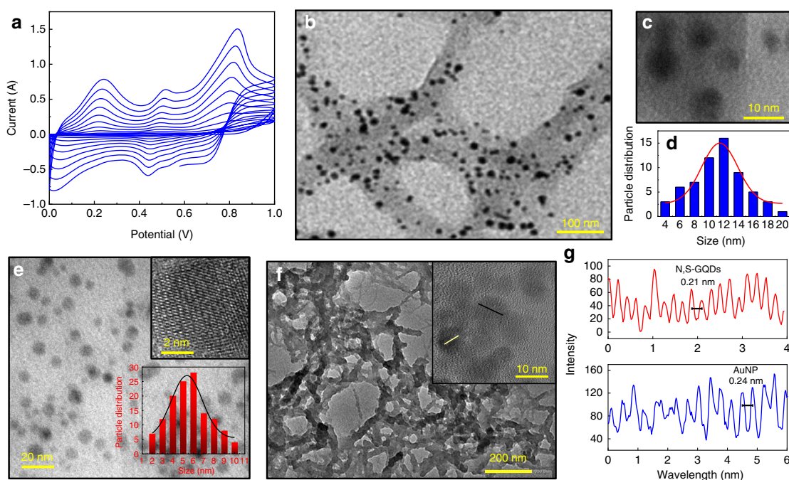
Fig. 2 Characterizations of polyaniline deposition, N,S-GQDs and Au-PAni preparation and N,S-GQDs@AuNP-PAni nanocomposites: a cyclic voltammograms of electropolymerized PANi film on the GCE electrode, b TEM image of AuNP-PAni nanocomposites, c high magnification of AuNP on the PANi chain, d size distribution of the AuNPs inside the AuNP-PAni nanocomposites, e TEM image of N,S-GQDs (inset: HRTEM image of an isolated N,S-GQD and the size distribution), f TEM image of N,S-GQDs@AuNP-PAni nanocomposites (inset: HRTEM of a small area), and g fringe patterns of N,S-GQDs and AuNP from the HRTEM image of N,S-GQDs@AuNP-PAni nanocomposites
