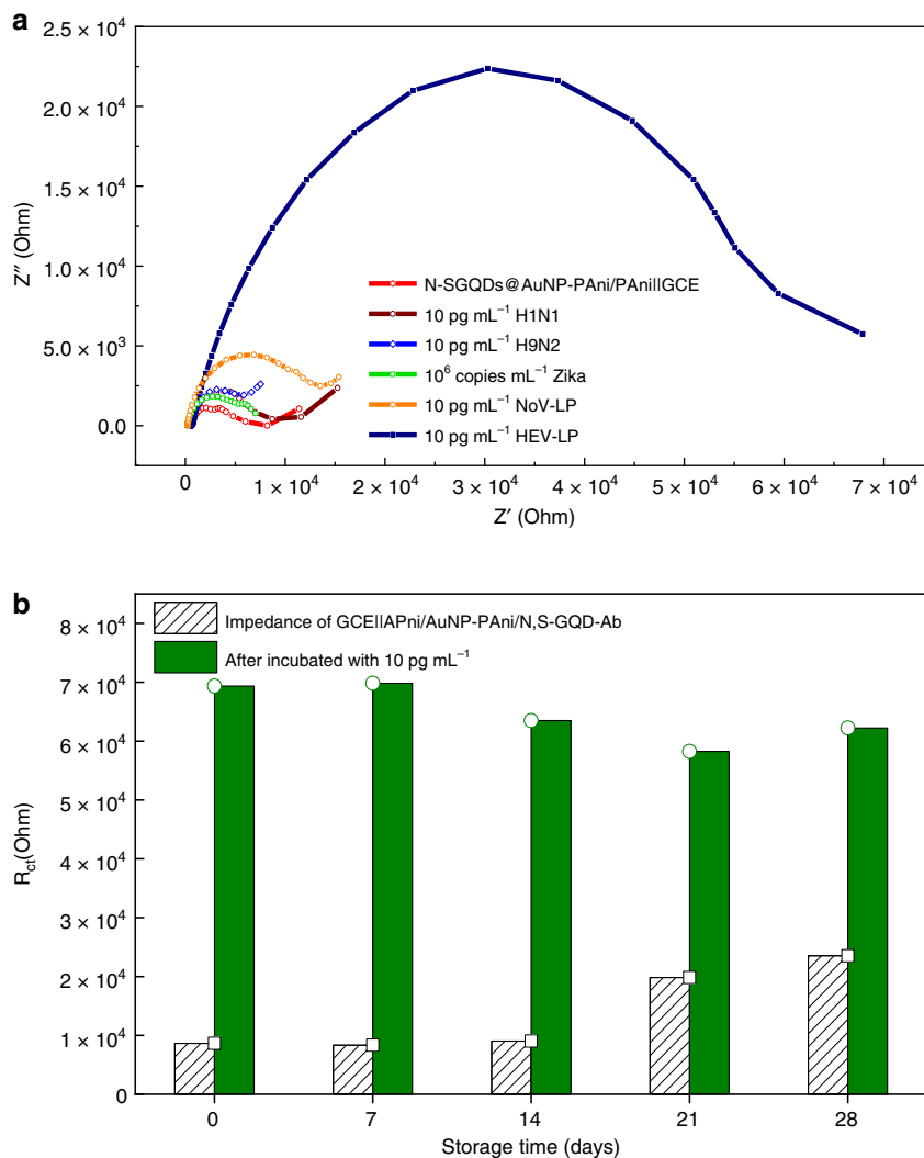
Fig. 6 Selectivity and stability of the proposed sensor. a Influenza virus A (H1N1 and H9N2), zika virus and NoV-LP were used for the selectivity test. b Stability of the GCE||PAni/AuNP-PAni/N,S-GQD-Ab electrode with (green bars) and without (shaded bars) 10 \text{ pg mL}^{-1} HEV-LP incubation over 4-week period
