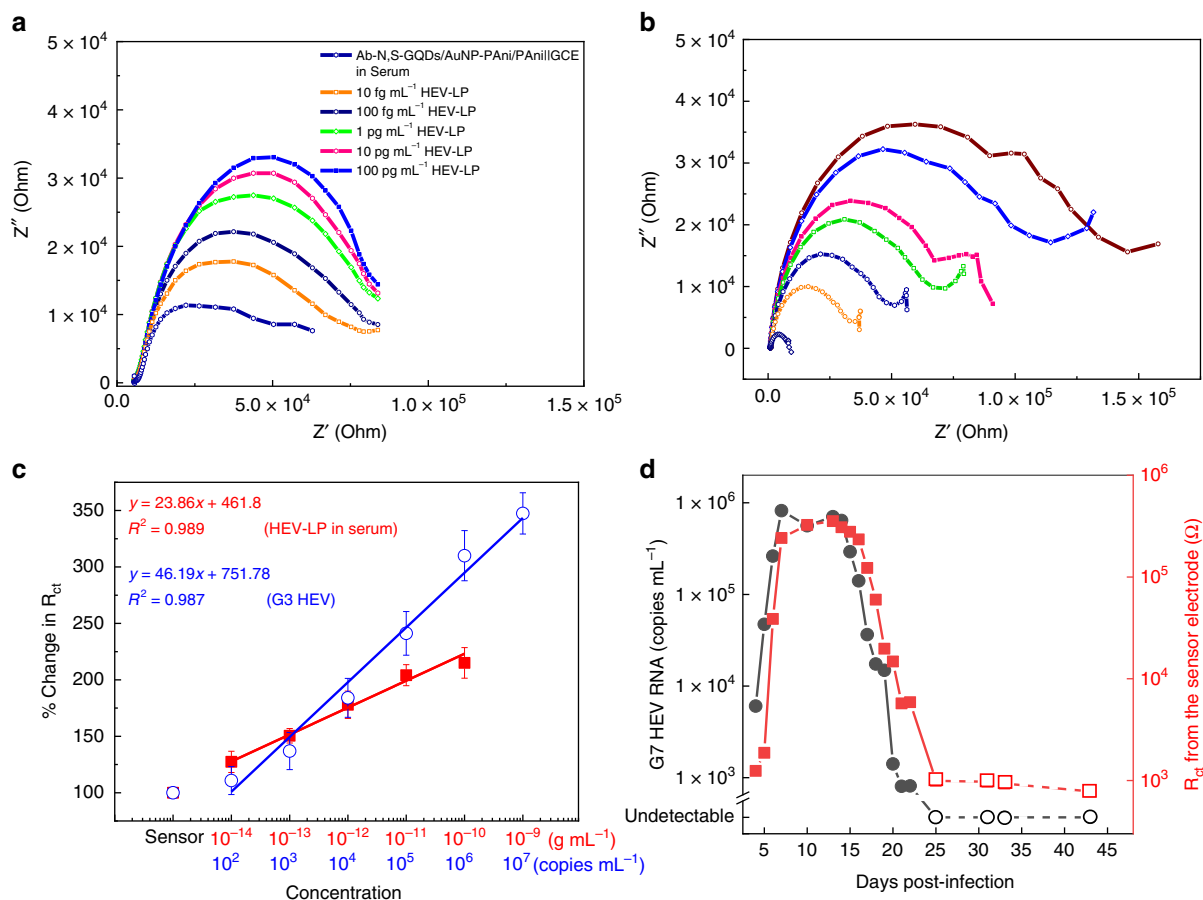
Fig. 7 Sensor performances in serum and different HEV analytes. Detection of HEV-LP in human serum ( a ) and G3 HEV in cell culture supernatants ( b ). c R_{ct} vs. HEV for both cases of HEV-LP (closed squares) in serum and G3 HEV (open circles) in cell culture supernatants. Error bars represent the standard deviation of triple measurements. d Comparison of the sensitivity between the impedimetric sensor (closed squares) and RT-qPCR (closed circles) by detection of G7 HEV in fecal specimens. The fecal specimens were collected at 4–43 dpi from an experimentally G7 HEV-infected cynomolgus macaque monkey. Open circles represent samples in which the viral RNAs are undetectable by RT-qPCR
