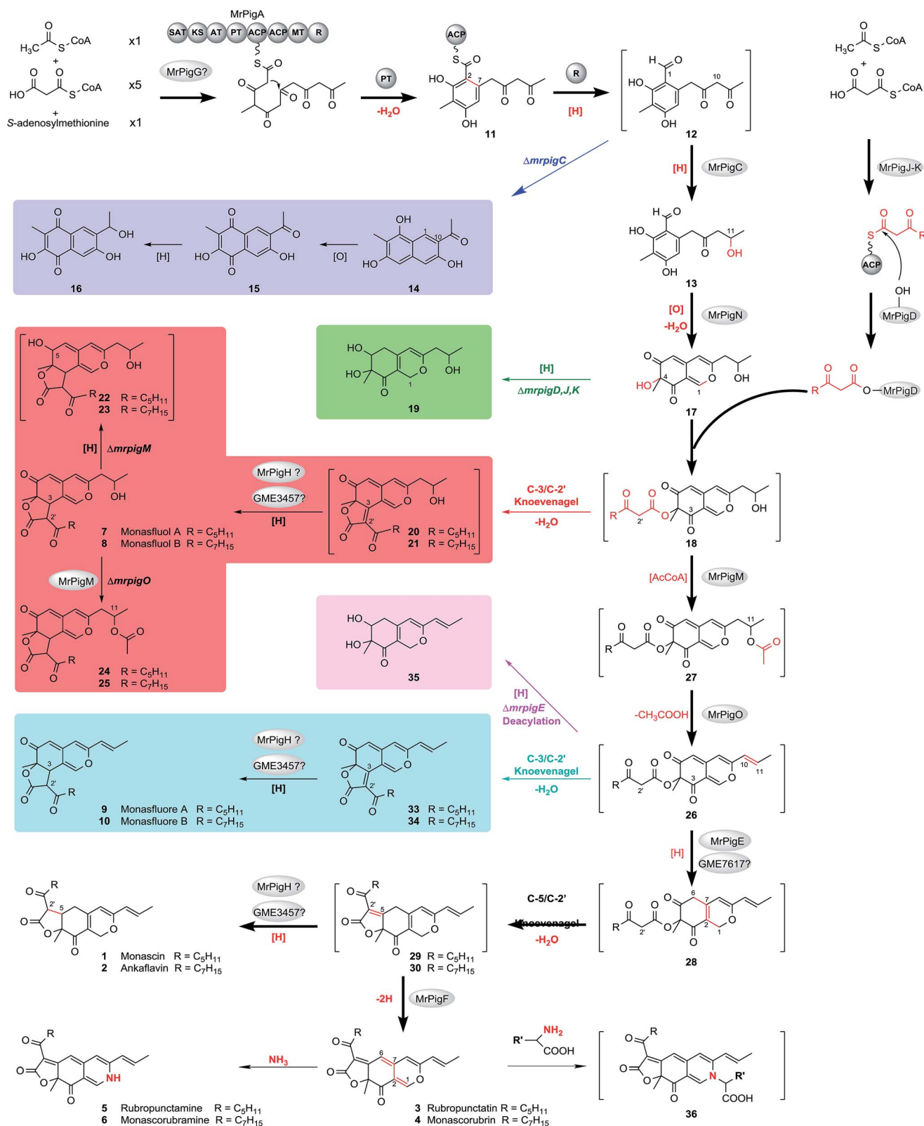
Scheme 2 Proposed biosynthetic pathway for MonAzPs in M. ruber M7. Yellow pigments: 1 , 2 , 7–10 , 13–17 , 19–25 , 29 , 30 , and 33–35 . Orange pigments: 3 , and 4 . Red pigments: 5 , 6 , and 36 . 36 is a model for amino acid derivatives of red MonAzPs. The spectral data is kept in ESI† Sections 6 and 9. 12 , 18 , and 26–28 are too reactive to isolate, whereas other compounds in square brackets were detected by MS but were not present in high enough concentration for NMR analysis. The main MonAzPs pathway is emphasized with bold arrows. Shunt pathways that contribute to the diversity of yellow pigments are boxed in color. See text for abbreviations. Red atoms and bonds indicate the chemical changes.
