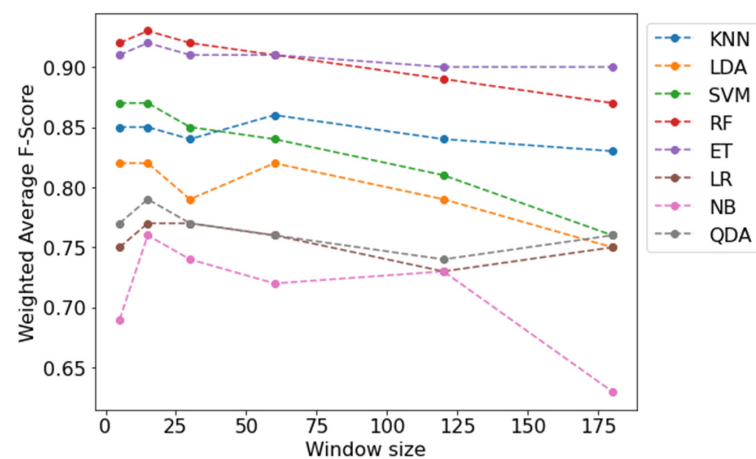
Figure 2. F-scores for each algorithm across all window lengths.
