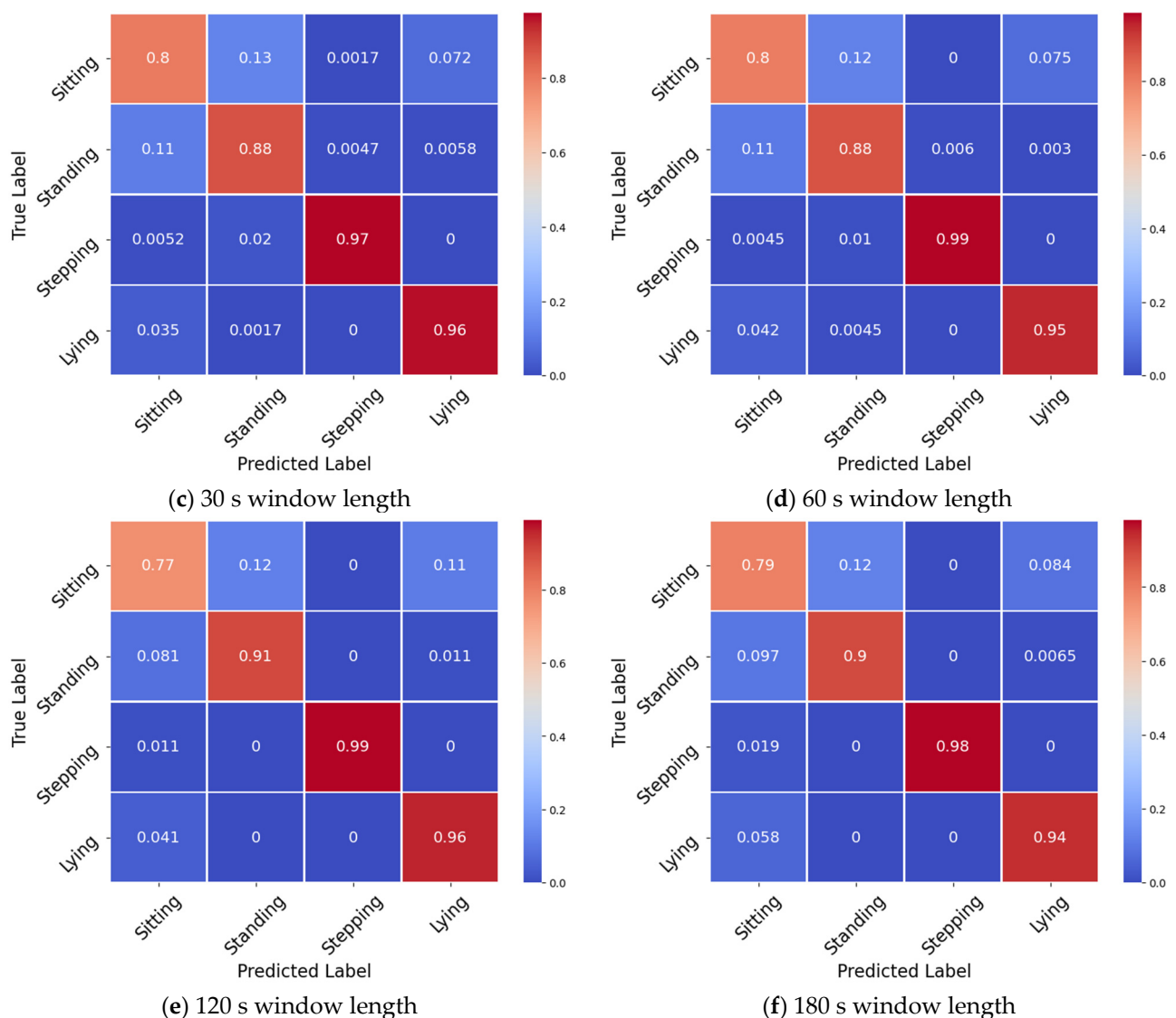
Figure 4. Confusion matrices for the RF classifier across the different window lengths: (a) 5, (b) 15, (c) 30, (d) 60, and (e) 120, (f) 180.
