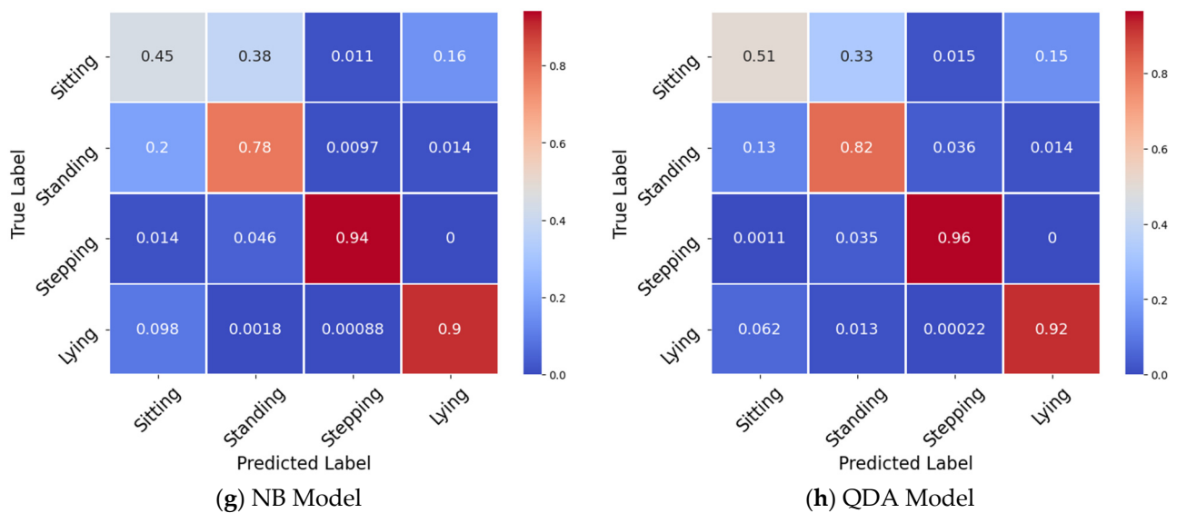
Figure 3. Confusion matrices for each classifier utilizing a 15 s window length: (a) KNN, (b) LDA, (c) SVM, (d) RF, (e) ET, (f) LR, (g) NB, and (h) QDA.
