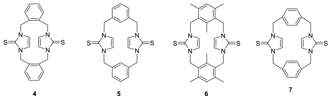
Fig. 2 Cyclophanes incorporating imidazole-2-thione moieties.
