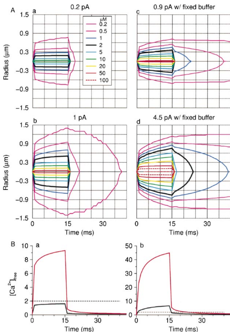
FIGURE 11. Simulations of spatiotemporal profile of Ca^{2+} concentration in response to a 15-ms pulse of Ca^{2+} current from a focal SR Ca^{2+} release site. Simulation of signal mass calculated from the total fluorescence in response to Ca^{2+} currents released from a focal SR source into the cytosol in the presence of 50 \mu M fluo-3 alone or in the presence of fixed buffer at a concentration of 230 \mu M , with a k_{on} of 10^{-8} M^{-1}s^{-1} and k_{off} of 200 s^{-1} . See also Fig. 1. The Ca^{2+} currents used (0.2 and 1 pA in the absence of fixed buffer, and 0.9 pA and 4.5 pA in its presence) are based on measured values of the signal mass. In each case, the concentration changes shown result from a 15-ms pulse of Ca^{2+} current (not shown). (A) Spatiotemporal profiles of [Ca^{2+}] in response to a 15-ms pulse of current of the magnitude indicated and with onset at time 0 in the absence (a, 0.2 pA; and b, 1 pA) and the presence (c, 0.9 pA; and d, 4.5 pA) of fixed buffer. (B) Time course of change in [Ca^{2+}] at a fixed distance (200 nm) from the release site in response to a 15-ms pulse of Ca^{2+} current in the absence (a, black line for 0.2 pA; and red line for 1 pA) and the presence (b, black line for 0.9 pA; and red line for 4.5 pA) of fixed buffer. The dashed line indicates the [Ca^{2+}]_{EC50} for the BK channels in excised patches at 0 mV.
