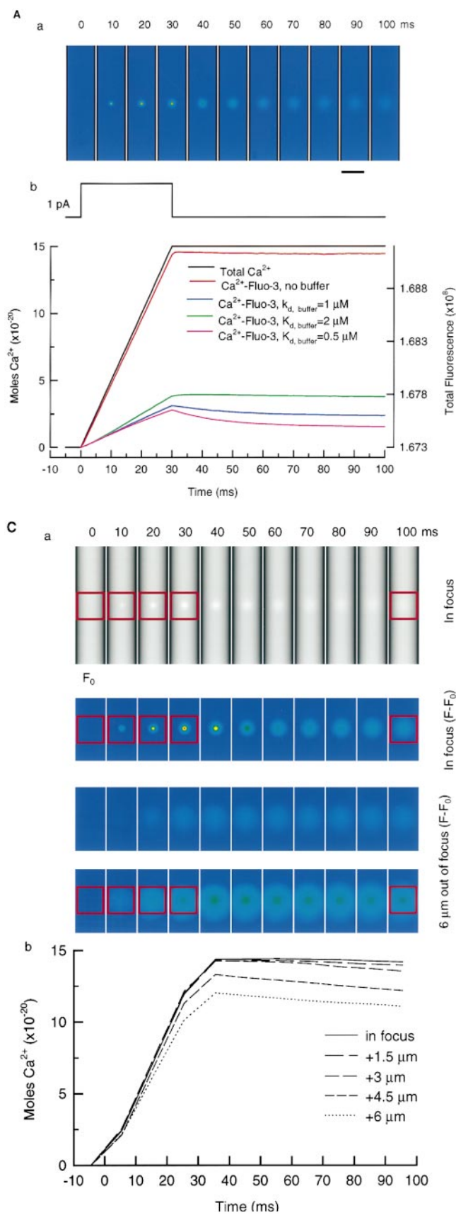
FIGURE 1. Computer simulation of \text{Ca}^{2+} entry into the cytosol reveals that the increase in total fluo-3 fluorescence (i.e., signal mass) is a reliable indicator of the total quantity of \text{Ca}^{2+} released. (A) Reaction-diffusion kinetics of fluo-3 were simulated in response to a \text{Ca}^{2+} current (1 pA in magnitude and 30 ms in duration; top panel of b) from a point source into the center of a cylindrical model cell with a diameter of 12 \mu\text{m} . a shows the evolution of a continuous series of simulated 10-ms fluorescence images. The bottom panel of b shows the integrated \text{Ca}^{2+} , i.e., the signal mass (black line), and the total increase in fluorescence emitted from \text{Ca}^{2+} -bound fluo-3 under various conditions: in the absence of fixed buffers (red line) and in the presence of 230- \mu\text{M} fixed \text{Ca}^{2+} buffer with a K_d of 0.5 \mu\text{M} (pink line), 1 \mu\text{M} (blue line), or 2 \mu\text{M} (green line). (In each case, the fixed buffer has the same k_{on} , appropriate for diffusion limitation and varying k_{off} 's.) Note that, in the absence of fixed buffer, fluo-3 fluorescence closely follows the change of total \text{Ca}^{2+} from the source, suggesting that most of the \text{Ca}^{2+} ions are bound to fluo-3; and that fixed buffers proportionally decrease fluo-3 fluorescence as their K_d increases. Parameters used for simulations are as follows: basal \text{Ca}^{2+} concentration of 0.1 \mu\text{M} ; total fluo-3 concentration of 50 \mu\text{M} and total endogenous fixed buffer concentration of 230 \mu\text{M} ; an on-rate of 8 \times 10^{-7} \text{ M}^{-1}\text{s}^{-1} for fluo-3 and 10^{-8} \text{ M}^{-1}\text{s}^{-1} for fixed buffer; an off-rate of 90 \text{s}^{-1} for fluo-3 and 50, 100, 200 \text{s}^{-1} for fixed buffer (yielding a K_d of 1.1 \mu\text{M} for fluo-3 and 2, 1, 0.5 \mu\text{M} , respectively, for fixed buffers); a diffusion constant of 250 \mu\text{m}^2\text{s}^{-1} for \text{Ca}^{2+} and 22 \mu\text{m}^2\text{s}^{-1} for free fluo-3. (B) Results of simulations like the ones in Fig. 1 A, showing the amount of \text{Ca}^{2+} bound to fluo-3 at the end of a 30-ms pulse of a range of \text{Ca}^{2+} currents. For each level of \text{Ca}^{2+} current, the rise was linear with time as in Fig. 1 A. Top line (circles) gives the result in the presence of 50 \mu\text{M} fluo-3 alone, and the bottom line (squares) gives the result in the presence of both fluo-3 and 230 \mu\text{M} of 0.5 \mu\text{M} K_d fixed buffer illustrated in Fig. 1 A. This plot provides a calibration for the signal mass for a wide range of \text{Ca}^{2+} currents. (C) The measure of signal mass based on the wide-field microscope accounts for nearly all the fluorescence, whether the spark release site is in or out of focus. The fluorescence generated by the simulation shown in A was blurred in three dimensions using a PSF that was determined empirically as explained in Carington et al. (1995). The result is shown in the top row of a; note that this simulation is for a spark whose epicenter lies in the plane of microscope focus. The second row from the top displays the fluorescence above baseline for the data in the first row. The third row displays the fluorescence when the spark epicenter is out of focus at the same gain as the second row. The bottom row displays the same
