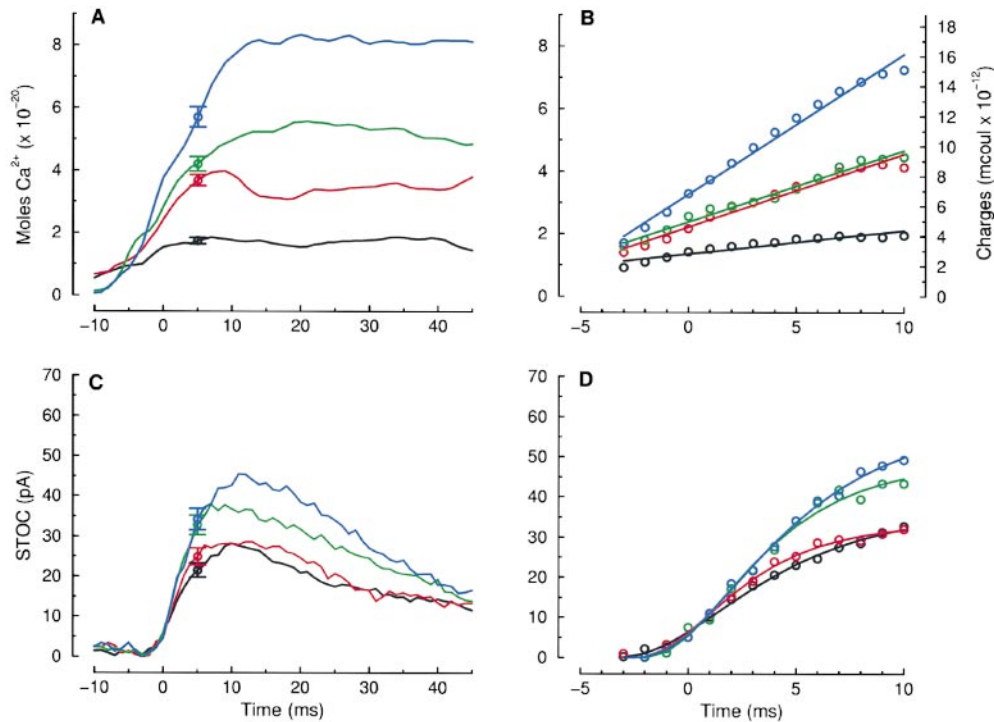
FIGURE 5. Mean I_{Ca(spark)} varies more than fivefold. (A) The averaged record for each of four groups of sparks arranged from smallest to largest. 146 individual sparks were ranked based on peak amplitude of their signal mass, and then divided into quarters, from smallest to largest. Sparks within each group were aligned and averaged according to the approach illustrated for a smaller number of events in Fig. 4 (i.e., the temporal alignment within each group is based on the corresponding STOCs). (B) Determination of the mean I_{Ca(spark)} from the slope of the initial rise of the signal mass traces in A. On the right vertical axis, the signal mass is converted to total charge. The slopes (i.e., mean I_{Ca(spark)} ) were 0.15, 0.44, 0.44, and 0.87 pA for the four groups from smallest to largest.
