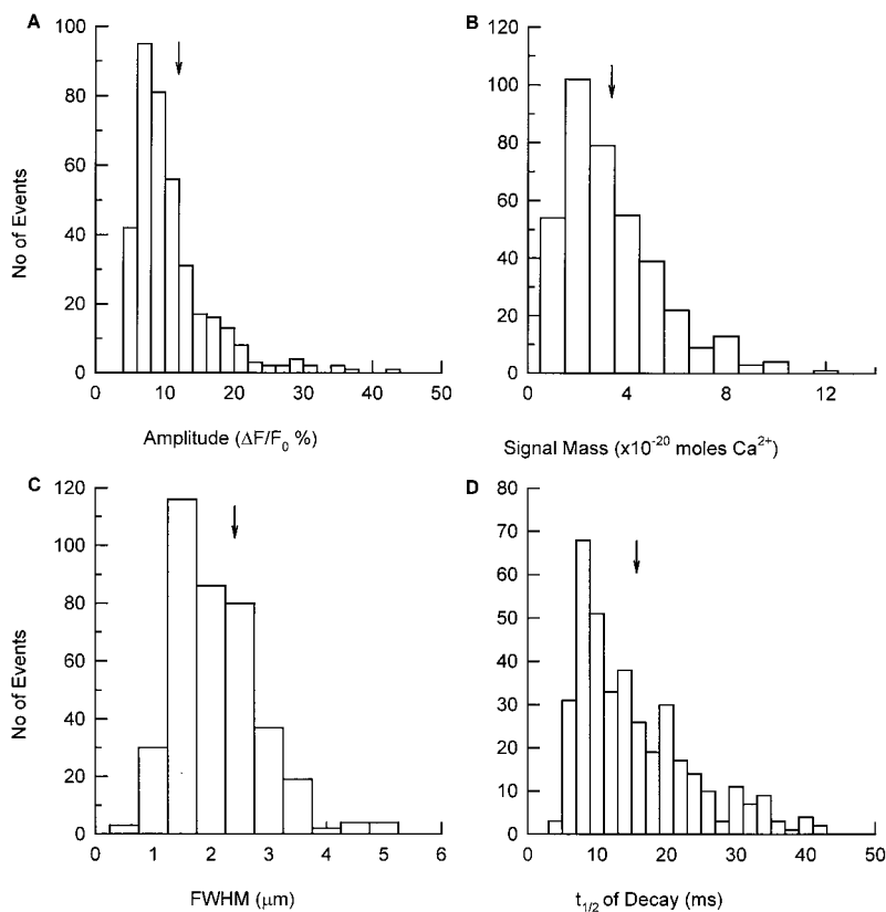
FIGURE 3. Histograms of \text{Ca}^{2+} spark amplitude, signal mass, full width at half maximum (FWHM), and t_{1/2} of decay. 365 \text{Ca}^{2+} sparks from 31 cells that were identified based on criteria described in the MATERIALS AND METHODS are used to construct the plots. Arrows indicate the mean of the distribution for each parameter. Values of mean \pm SEM are as follows: 11.6 \pm 0.29\% for \text{Ca}^{2+} spark amplitude; 3.4 \pm 0.1 \times 10^{-20} mol \text{Ca}^{2+} for signal mass; 2.4 \pm 0.04 \mu\text{m} for FWHM; and 16 \pm 0.45 ms for t_{1/2} of decay. Except for the signal mass, all measurements are based on \Delta\text{F}/\text{F}_0 at the epicenter pixel.
