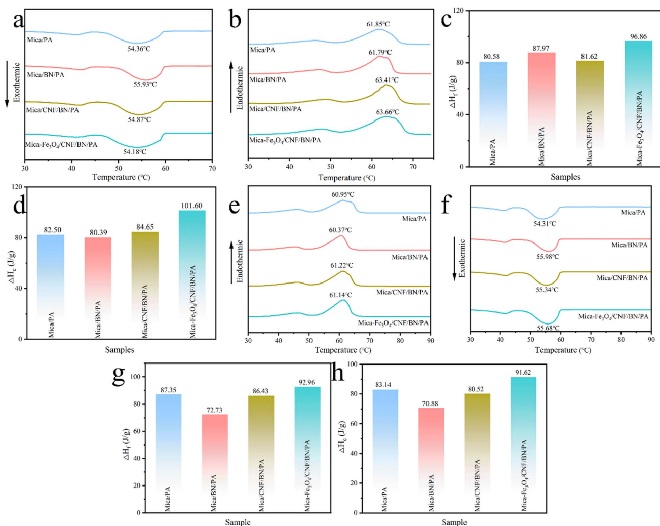
Fig. 5 (a) and (b) DSC of CPCMs, (c) melting enthalpy, (d) crystallization enthalpy, (e) and (f) DSC of CPCMs after 50 thermal cycling tests, (g) and (h) melting and crystallization enthalpy after 50 thermal cycling tests.
