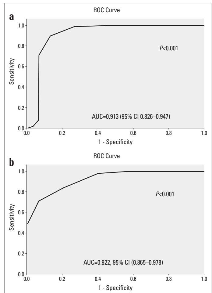
Figure 1. (a) The receiver operating characteristic curve for carotid intima-media thickness (CIMT) to predict coronary artery disease in patients with chronic obstructive pulmonary disease. (b) The receiver operating characteristic curve for carotid intima-media thickness (CIMT) to predict coronary artery disease in patients without chronic obstructive pulmonary disease
