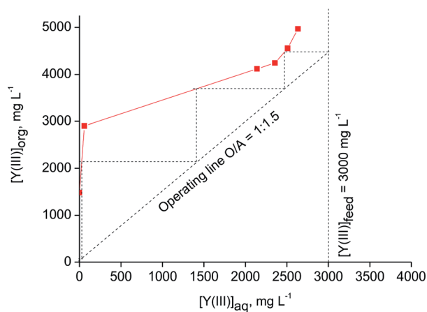
Fig. 5 McCabe–Thiele diagram for extraction of Y(III) with [C101][SCN] (aqueous phase: [\text{Y(III)}] = 3000 \text{ mg L}^{-1} , [\text{Eu(III)}] = 215 \text{ mg L}^{-1} , [\text{CaCl}_2] = 3 \text{ mol L}^{-1} , [\text{NH}_4\text{SCN}] = 0.2 \text{ mol L}^{-1} , T = 30 \text{ }^\circ\text{C} ).
