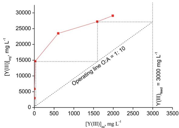
Fig. 6 McCabe–Thiele diagram for extraction of Y(III) with [C101][SCN] (aqueous phase: [\text{Y(III)}] = 3000 \text{ mg L}^{-1} , [\text{Eu(III)}] = 215 \text{ mg L}^{-1} , [\text{CaCl}_2] = 3 \text{ mol L}^{-1} , [\text{NH}_4\text{SCN}] = 0.8 \text{ mol L}^{-1} , T = 30 \text{ }^\circ\text{C} ).
